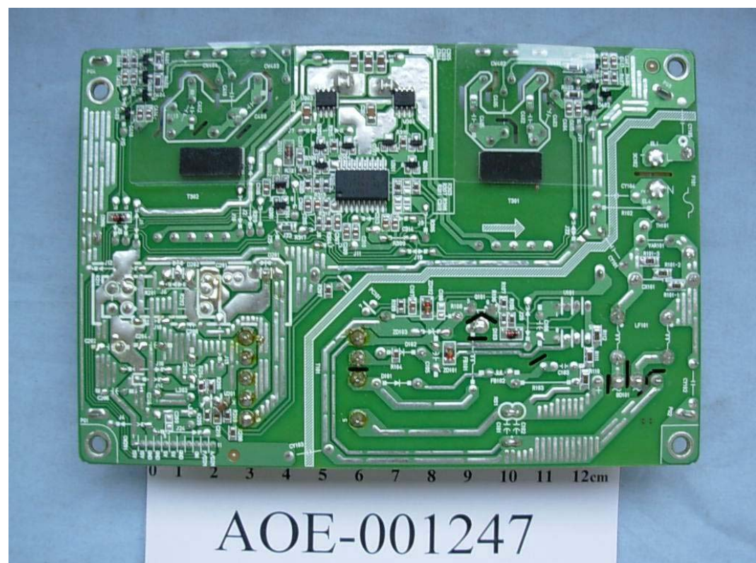
FIGURE 10 LCD MONITOR (M/N: L206WTQ) POWER BOARD (SOLDERED SIDE)
