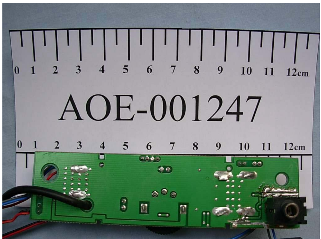
FIGURE 25 LCD MONITOR (M/N: L206WTQ) SPEAKER MAIN BOARD (BACK VIEW)
