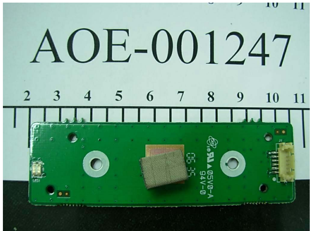
FIGURE 4 LCD MONITOR (M/N: L206WTQ) SWITCH BOARDS REMOVED (BACK VIEW)
