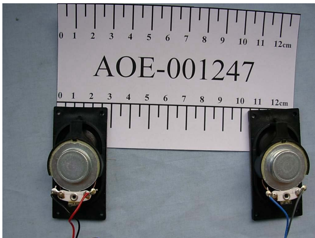
FIGURE 27 LCD MONITOR (M/N: L206WTQ) TRUMPET (BACK VIEW)
