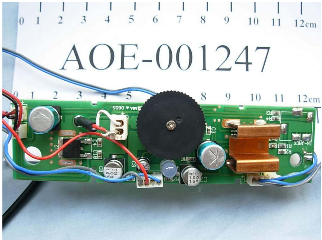
FIGURE 24 LCD MONITOR (M/N: L206WTQ) SPEAKER MAIN BOARD (FRONT VIEW)
