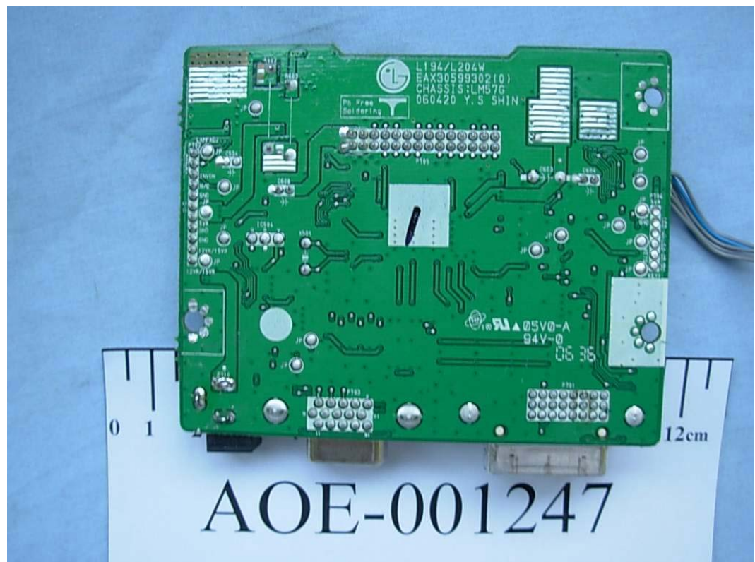
FIGURE 6 LCD MONITOR (M/N: L206WTQ) MAIN BOARD (SOLDERED SIDE)
