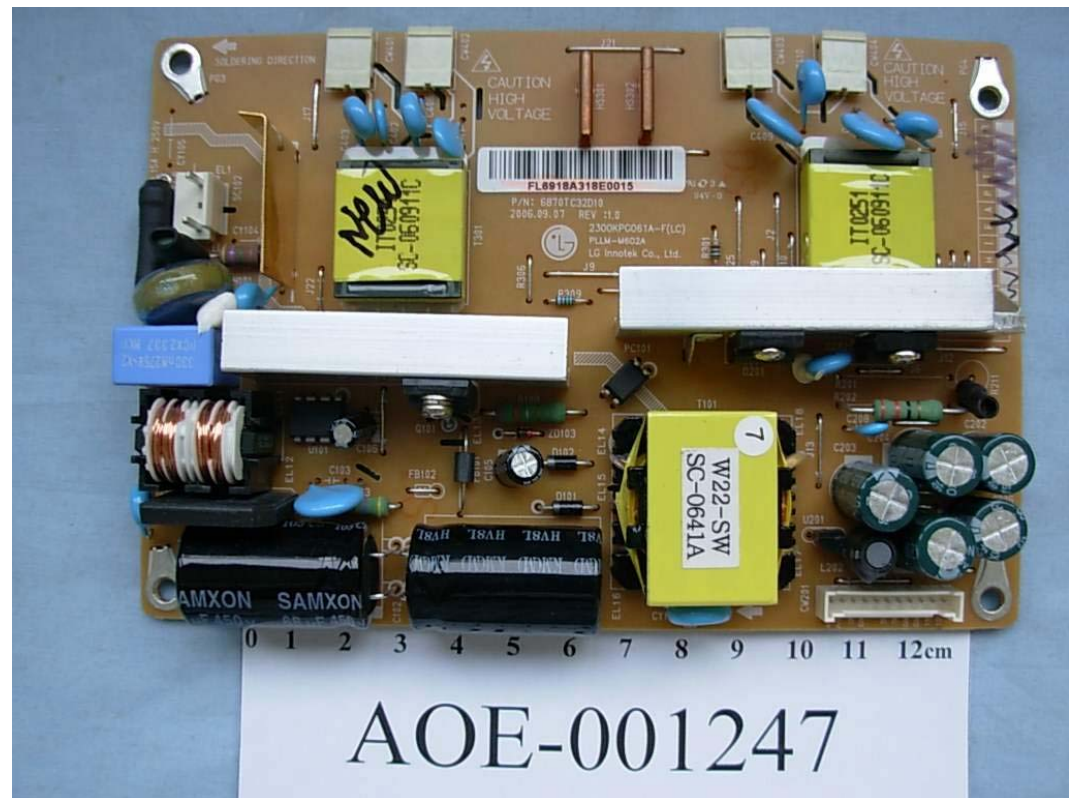
FIGURE 9 LCD MONITOR (M/N: L206WTQ) POWER BOARD (COMPONENT SIDE)
