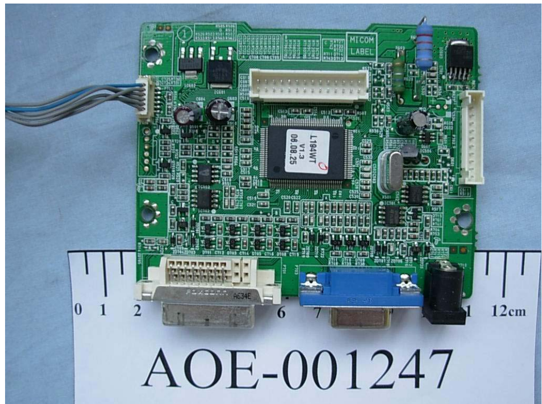
FIGURE 5 LCD MONITOR (M/N: L206WTQ) MAIN BOARD (COMPONENT SIDE)
