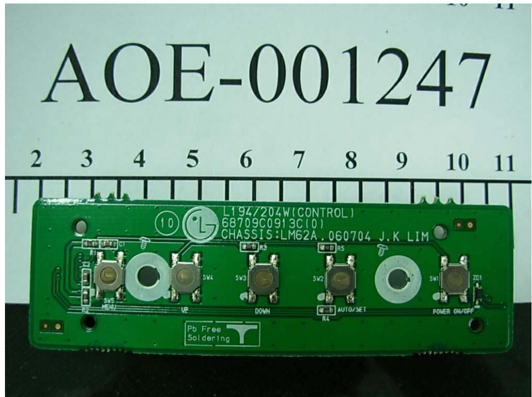
FIGURE 3 LCD MONITOR (M/N: L206WTQ) SWITCH BOARDS REMOVED (FRONT VIEW)
