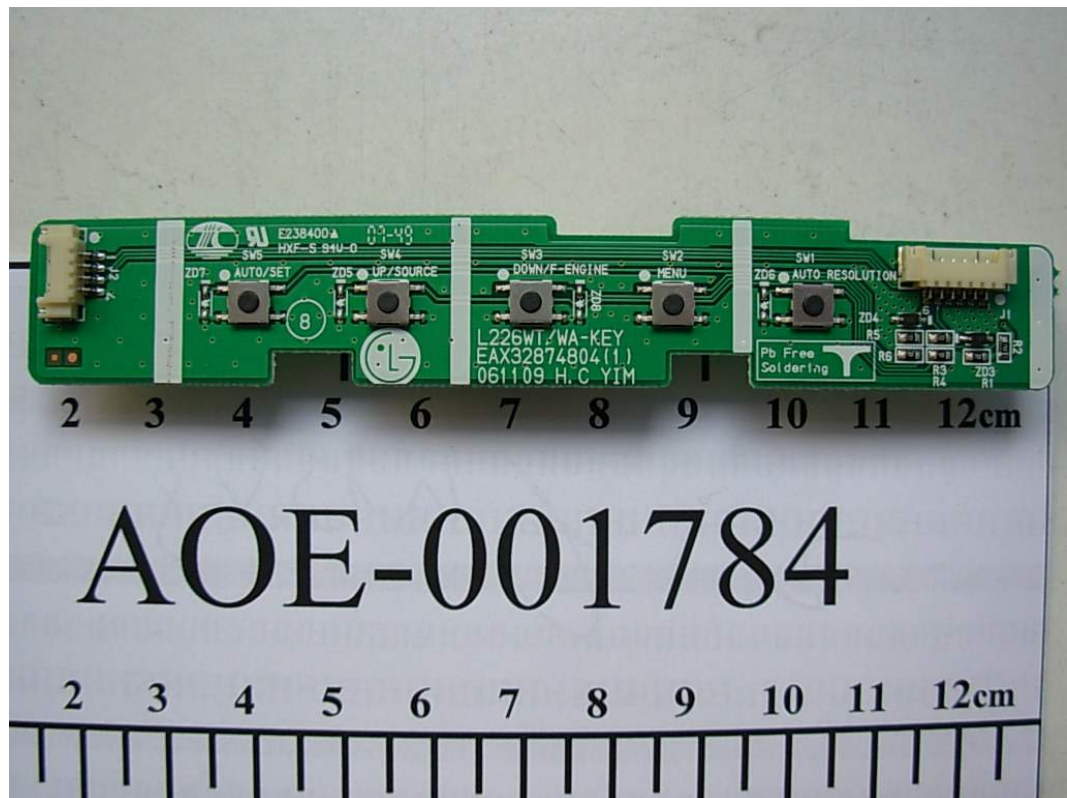
FIGURE 2 LCD MONITOR (M/N: L226WUQS) BUTTON BOARD (COMPONENT SIDE)
