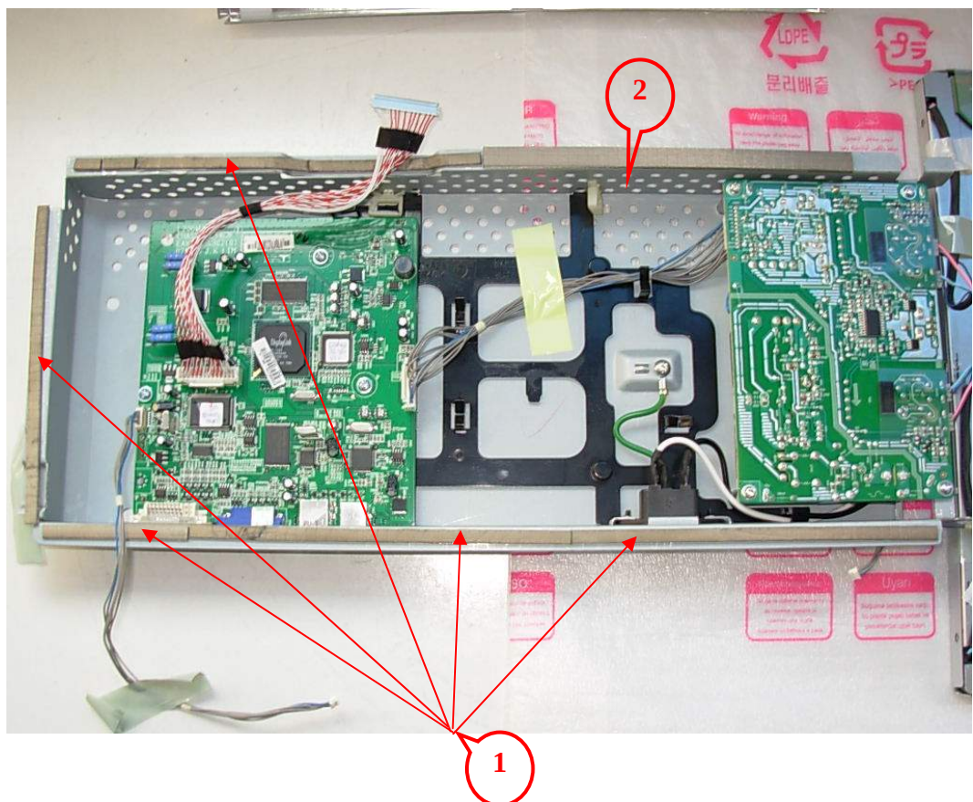
FIGURE 25 LCD MONITOR (M/N: L226WUQS) DEBUG #4
