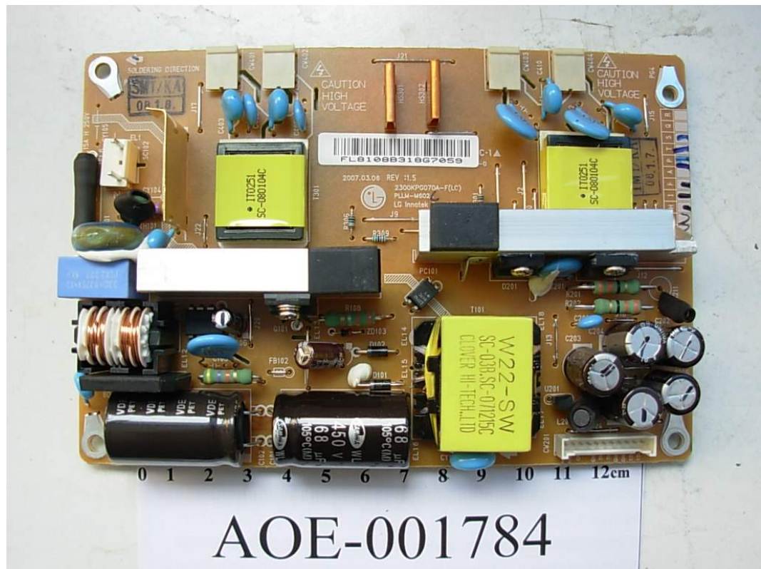
FIGURE 14 LCD MONITOR (M/N: L226WUQS) POWER BOARD (COMPONENT SIDE)
