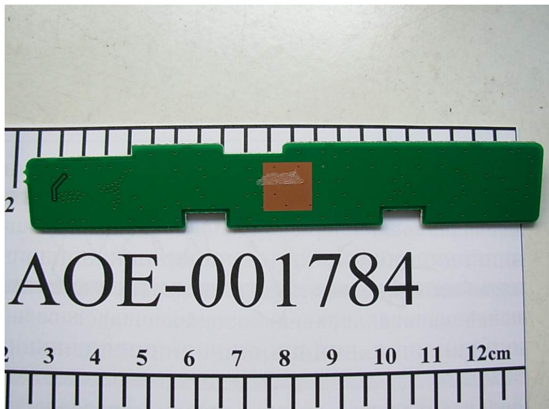
FIGURE 3 LCD MONITOR (M/N: L226WUQS) BUTTON BOARD (SOLDERED SIDE)
