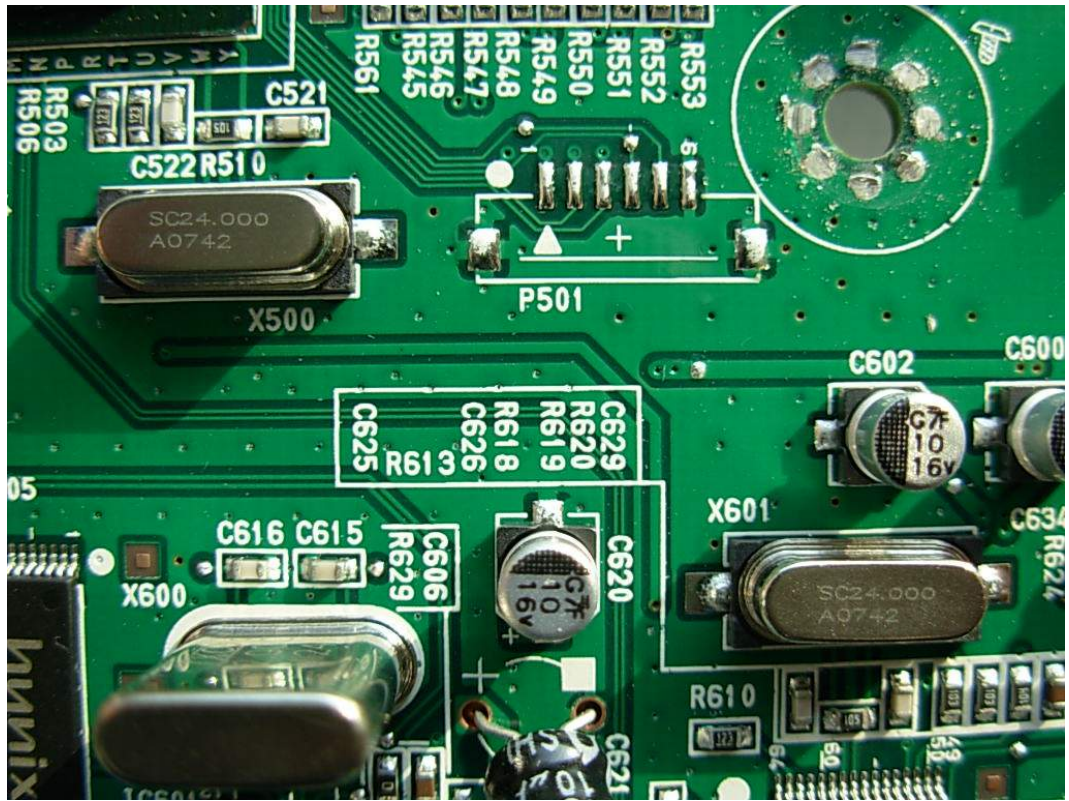
FIGURE 11 LCD MONITOR (M/N: L226WUQS) CRYSTAL #3 ON MAIN BOARD
