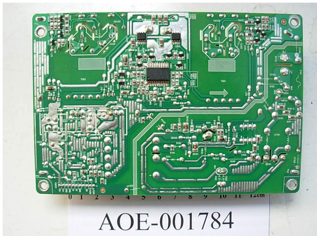
FIGURE 15 LCD MONITOR (M/N: L226WUQS) POWER BOARD (SOLDERED SIDE)
