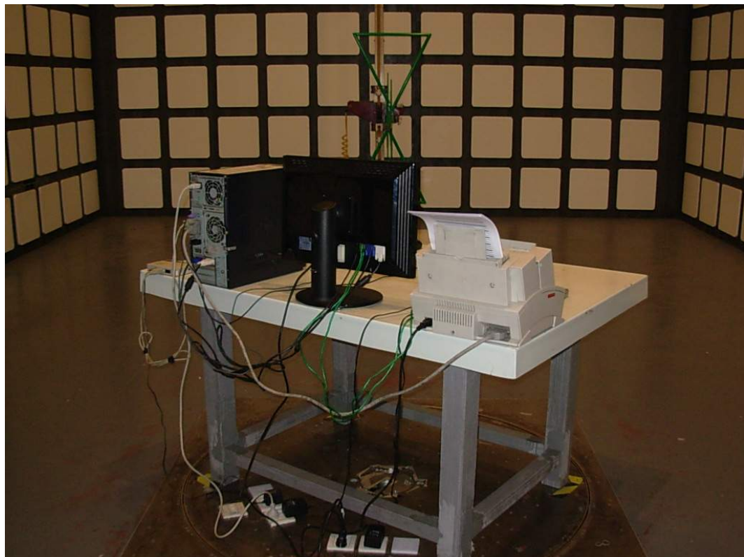
SETUP WITH MAXIMUM DETECTED EMISSION AT VERTICAL POLARIZATION (DVI 1680*1050@60Hz & USB CONNECTING)
