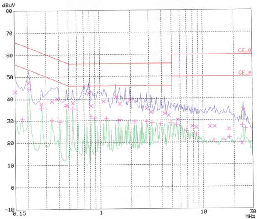
< Neutral line >
