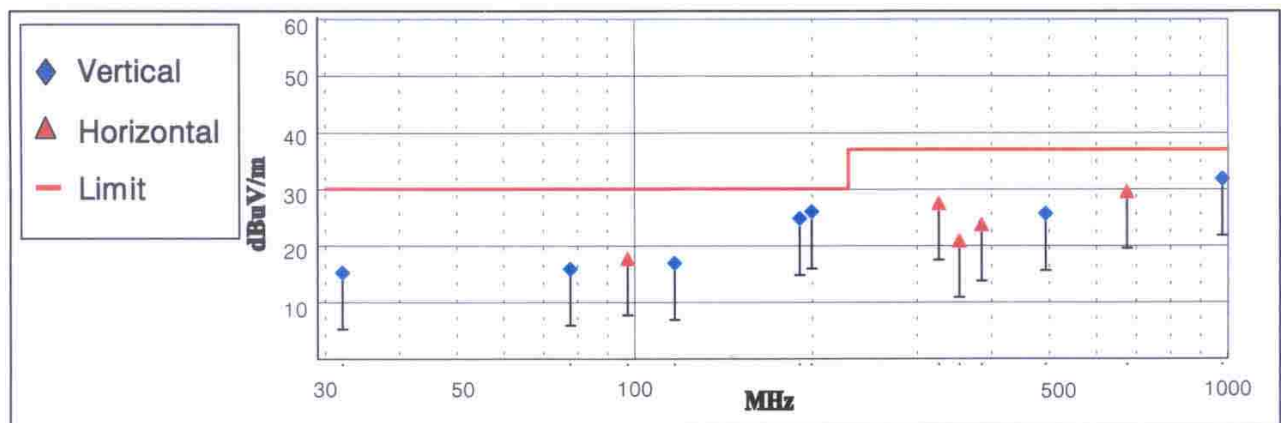
< Fig 4. Radiated emission result - Analog mode >
