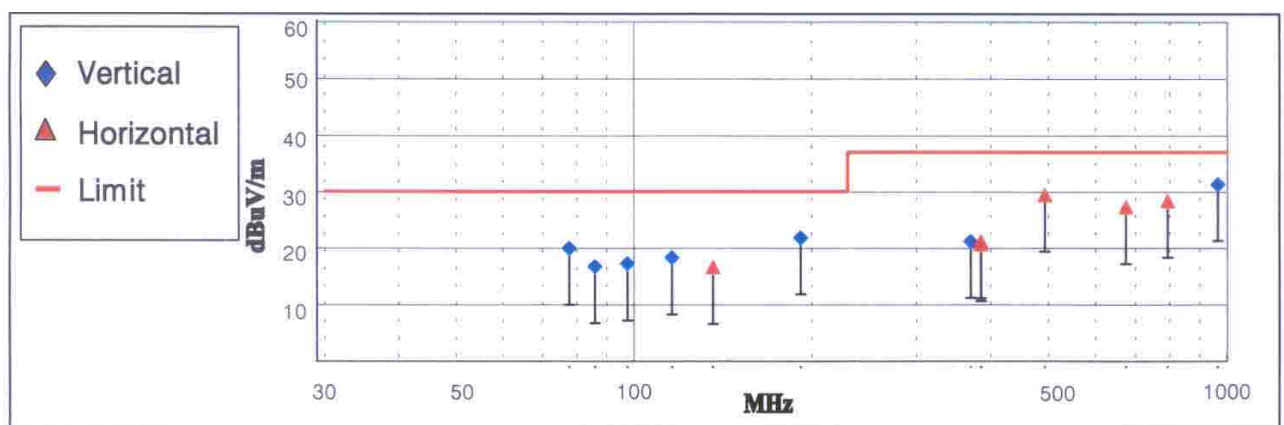
< Fig 5. Radiated emission result - Digital mode >
