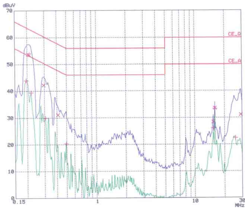
&lt; Neutral line &gt;
