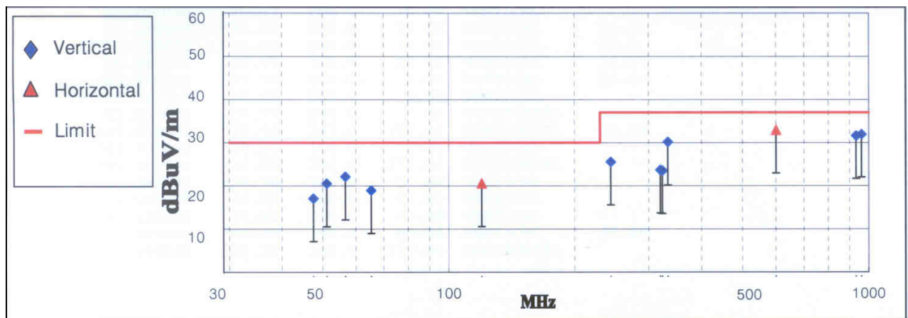
< Fig 6. Radiated Emission _ Digital(30MHz ~ 1000MHz) >
