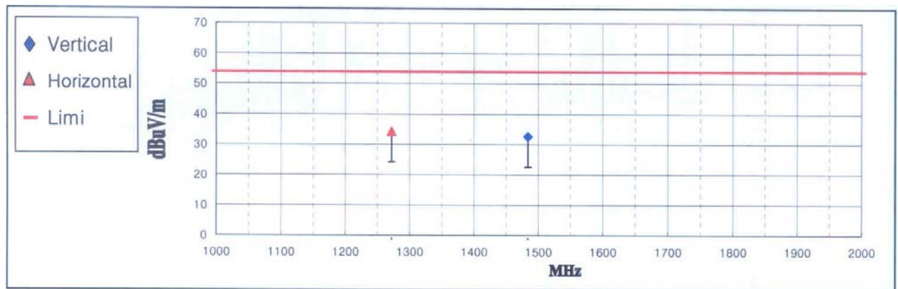
< Fig 7. Radiated Emission _ Digital(1000MHz ~ 2000MHz) >
