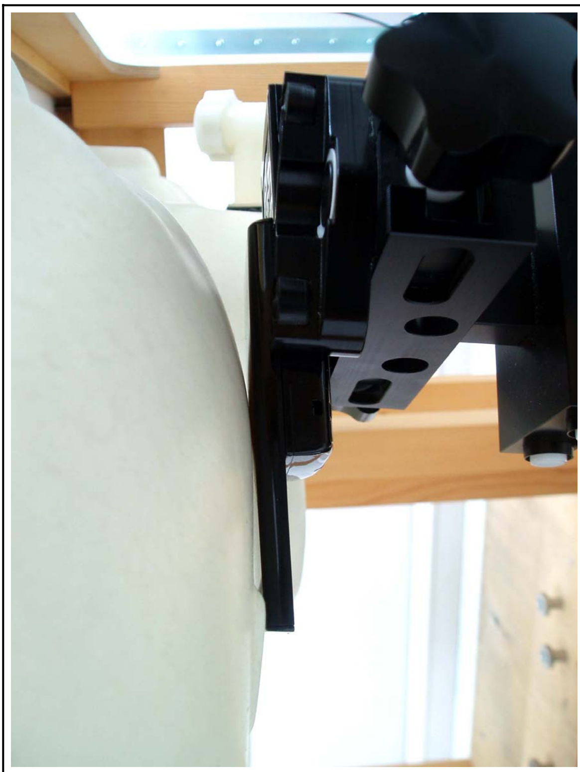
Figure 6 Right Head SAR Test Setup – Cheek Touch Position
