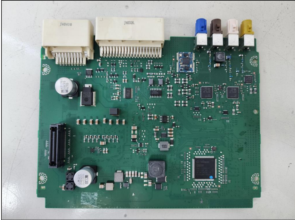
Bottom view of Sub PCB without shielding
