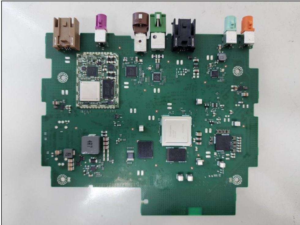
Top view of Main PCB without shielding
