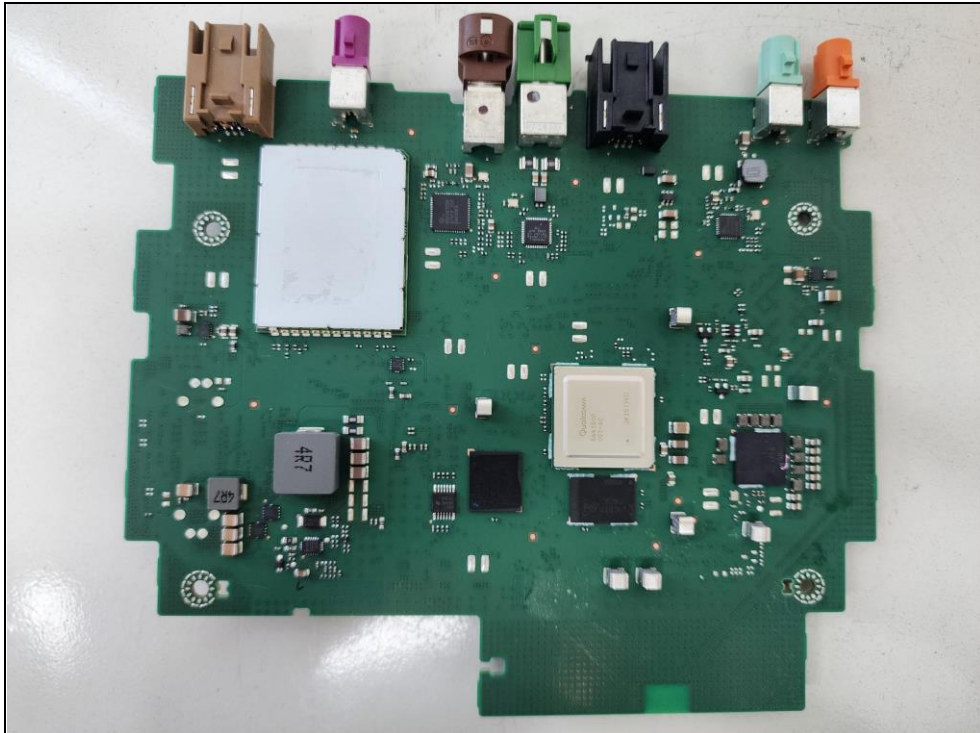
Top view of Main PCB with shielding
