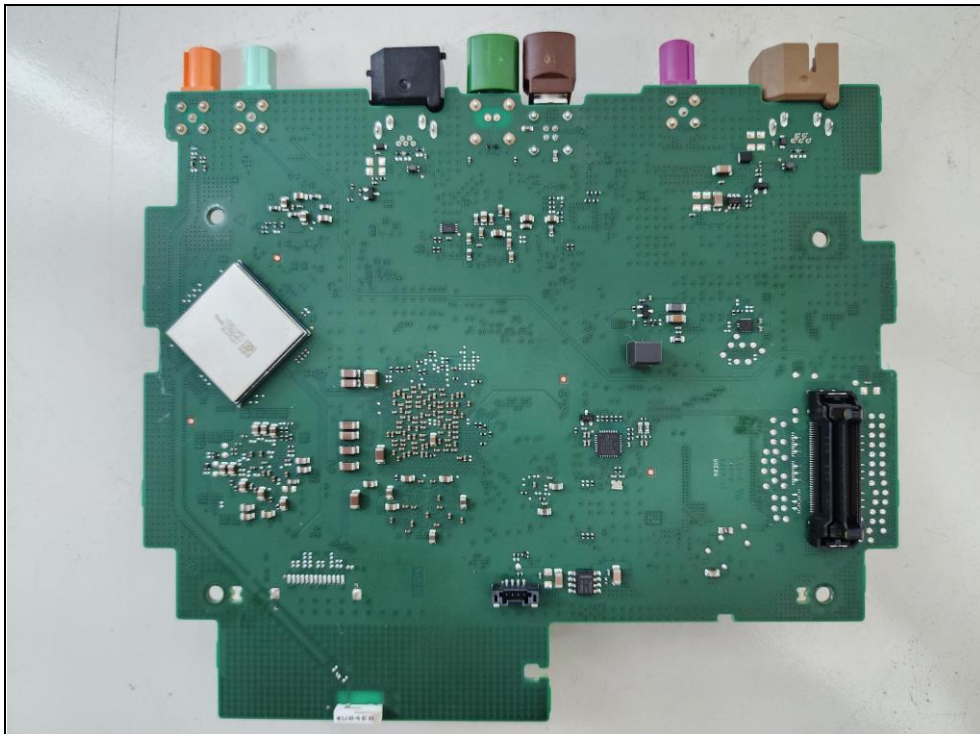
Bottom view of Main PCB with shielding
