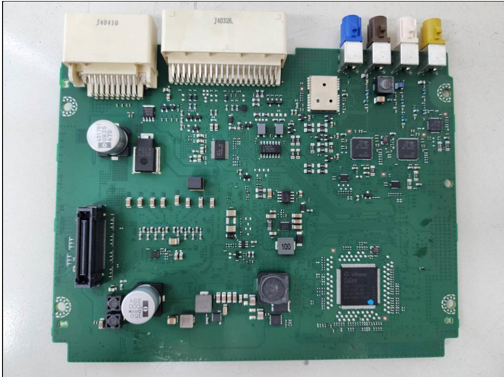
Top view of Sub PCB with shielding
