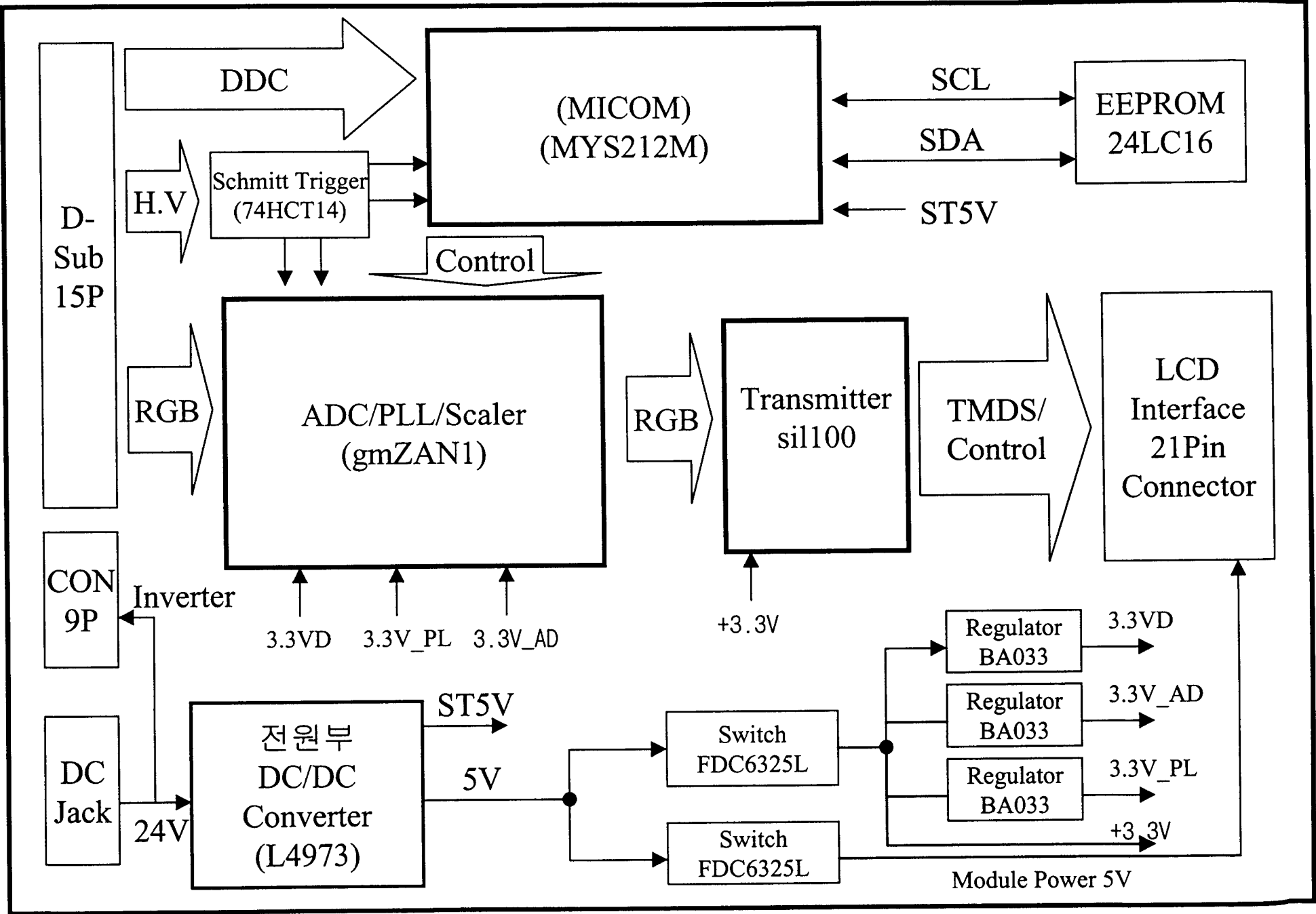
B563A Block Diagram
