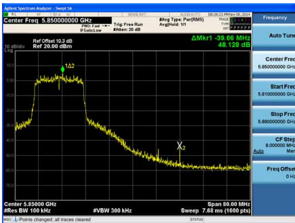
BandEdge (802.11a-CH 165)
