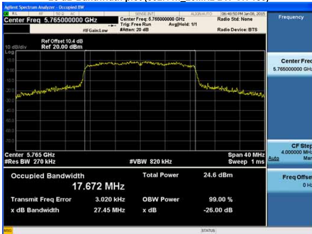
26 dB Bandwidth plot (802.11n_20MHz BW-CH 153)
