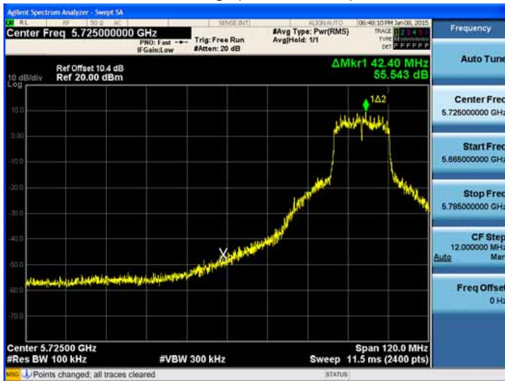
BandEdge (802.11a-CH 153)
