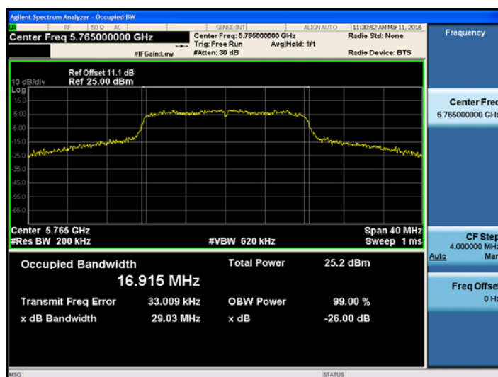
UNII 3 BAND 26dB Bandwidth (CH 153)
