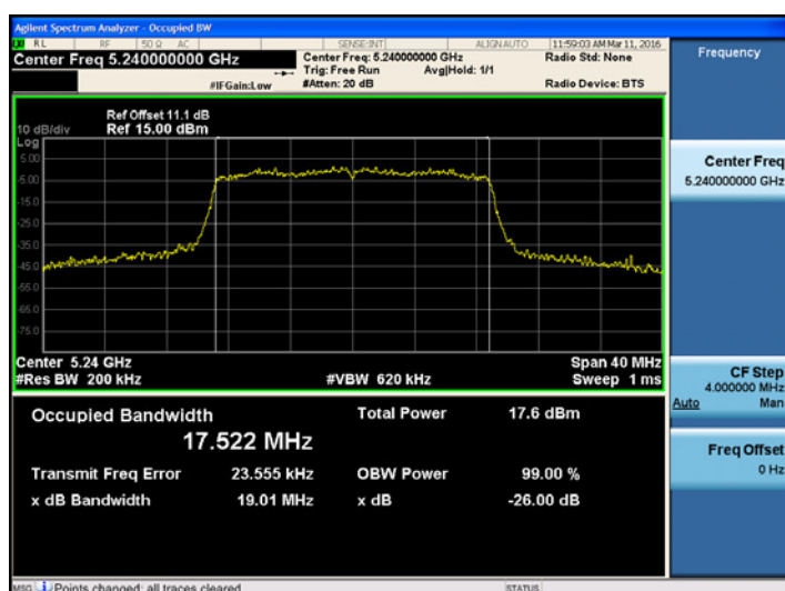
802.11n_20MHz UNII 1 BAND 99% Bandwidth (CH.48)
