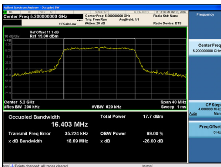
UNII 1 BAND 26dB Bandwidth (CH 40)
