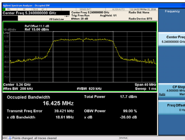
802.11a UNII 1 BAND 99% Bandwidth (CH.48)
