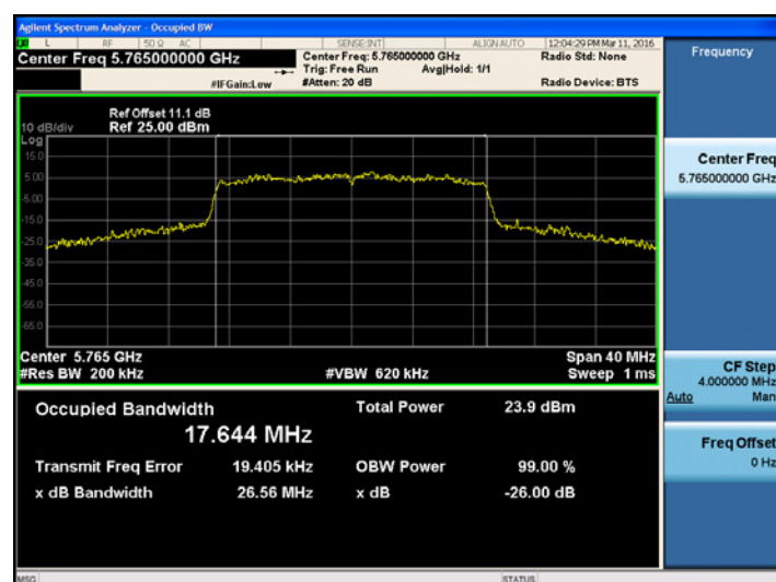
802.11n_20MHz UNII 3 BAND 99% Bandwidth(CH.153)
