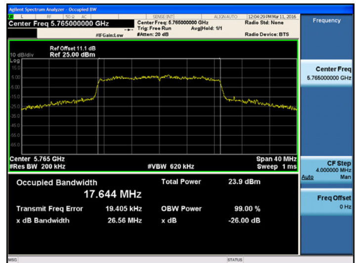
UNII 3 BAND 26dB Bandwidth (CH 153)
