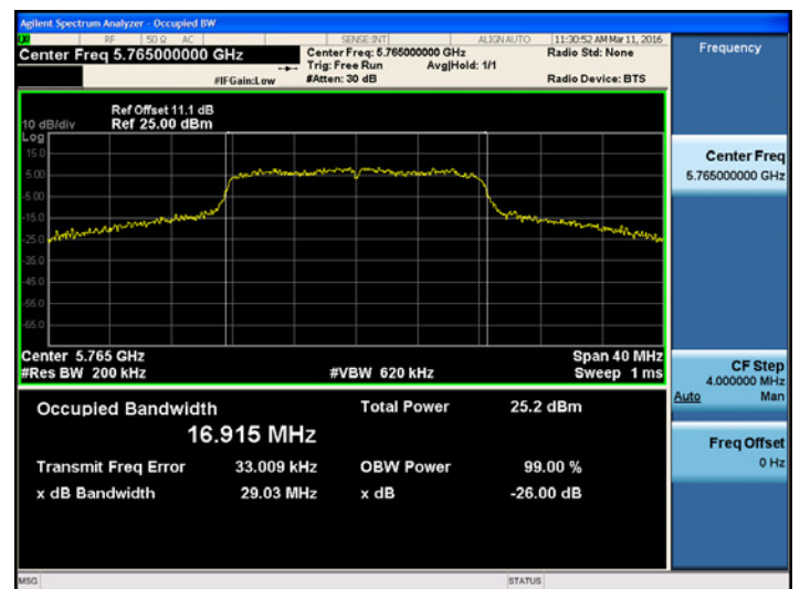
802.11a UNII 3 BAND 99% Bandwidth (CH.153)
