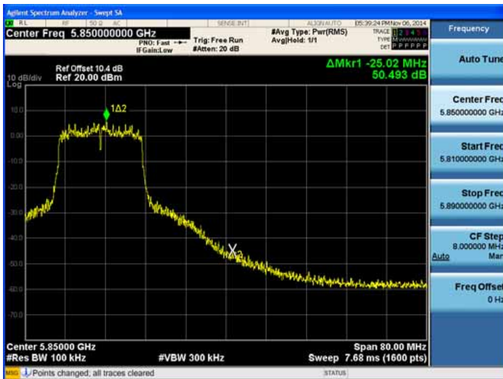
BandEdge (802.11a-CH 165)
