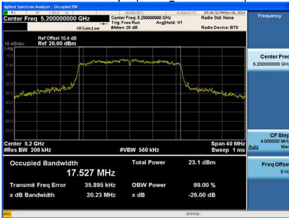
26 dB Bandwidth plot (802.11n_20MHz BW-CH 40)
