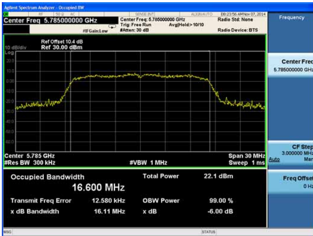
99% Bandwidth plot (802.11a-CH157)
