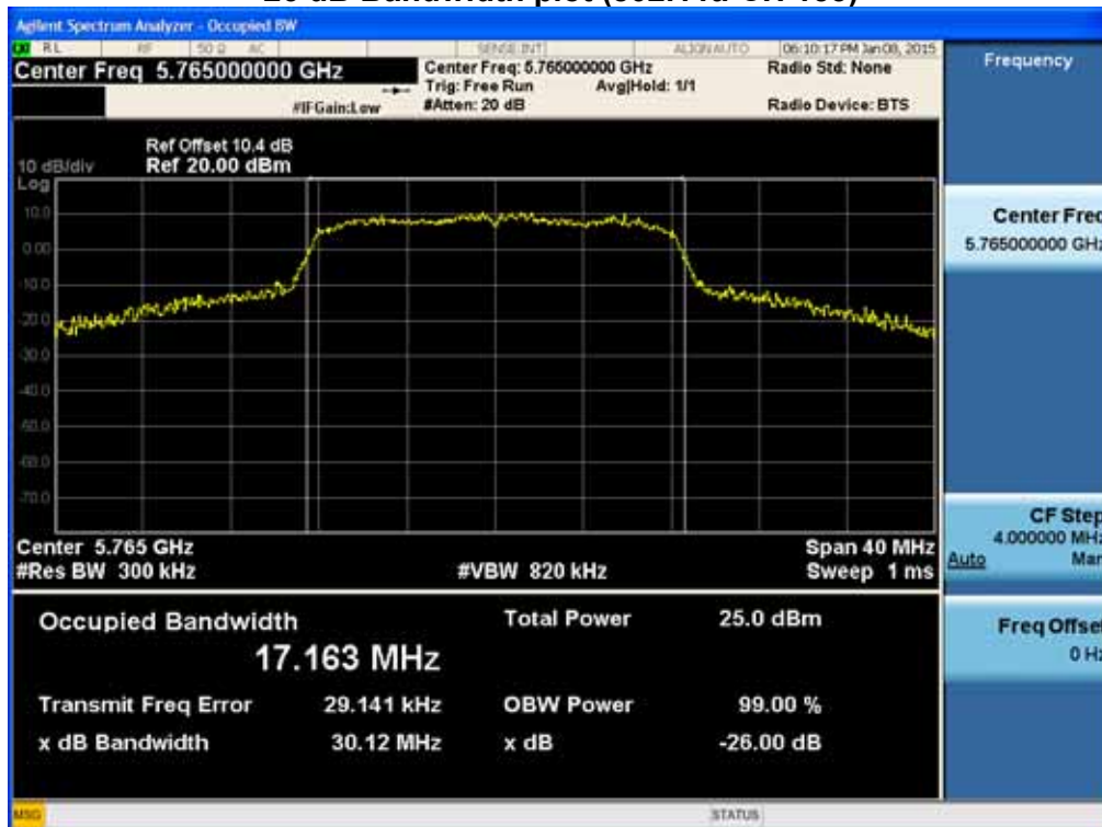
26 dB Bandwidth plot (802.11a-CH 153)
