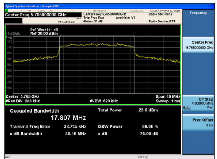
802.11n_HT20 UNII 3 BAND 99% Bandwidth(CH.153)
