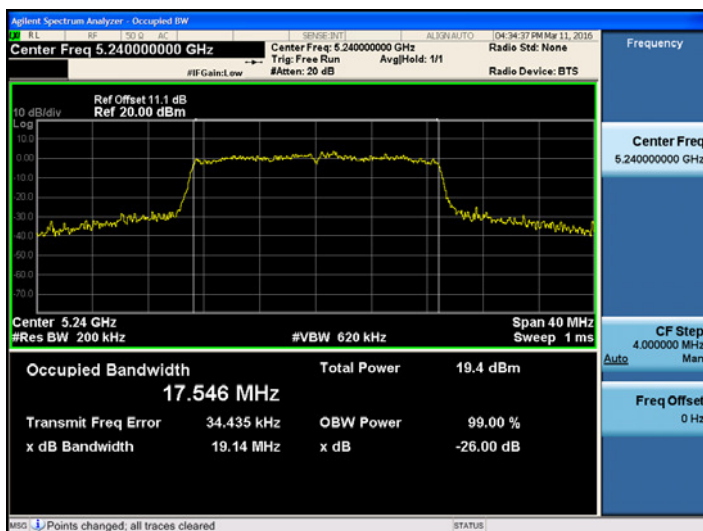
802.11n_HT20 UNII 1 BAND 99% Bandwidth (CH.48)
