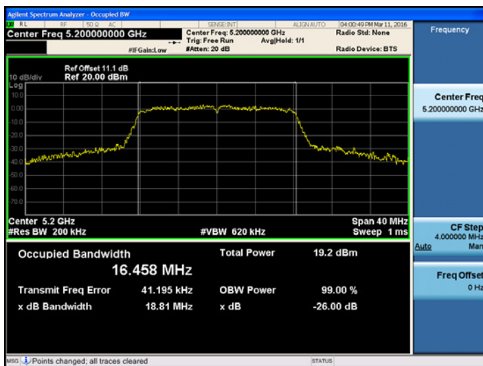
802.11a UNII 1 BAND 99% Bandwidth (CH.40)
