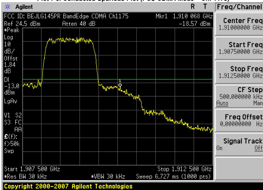
Plot 7-10. Band Edge Plot (PCS CDMA Mode – Ch. 1175)
