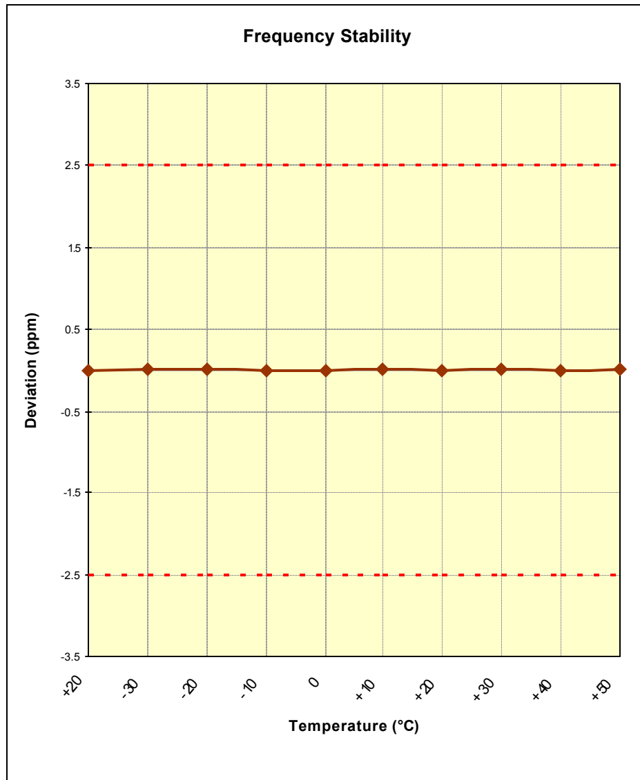
Figure 6-1. Frequency Stability Graph (PCS CDMA Mode – Ch. 600)
