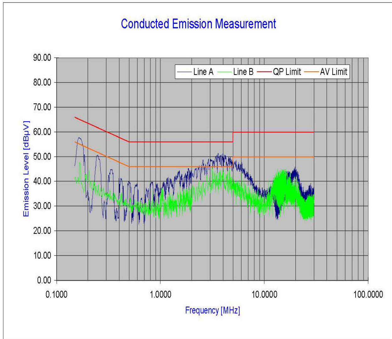
Plot 7-1. Line-Conducted Test Plot
