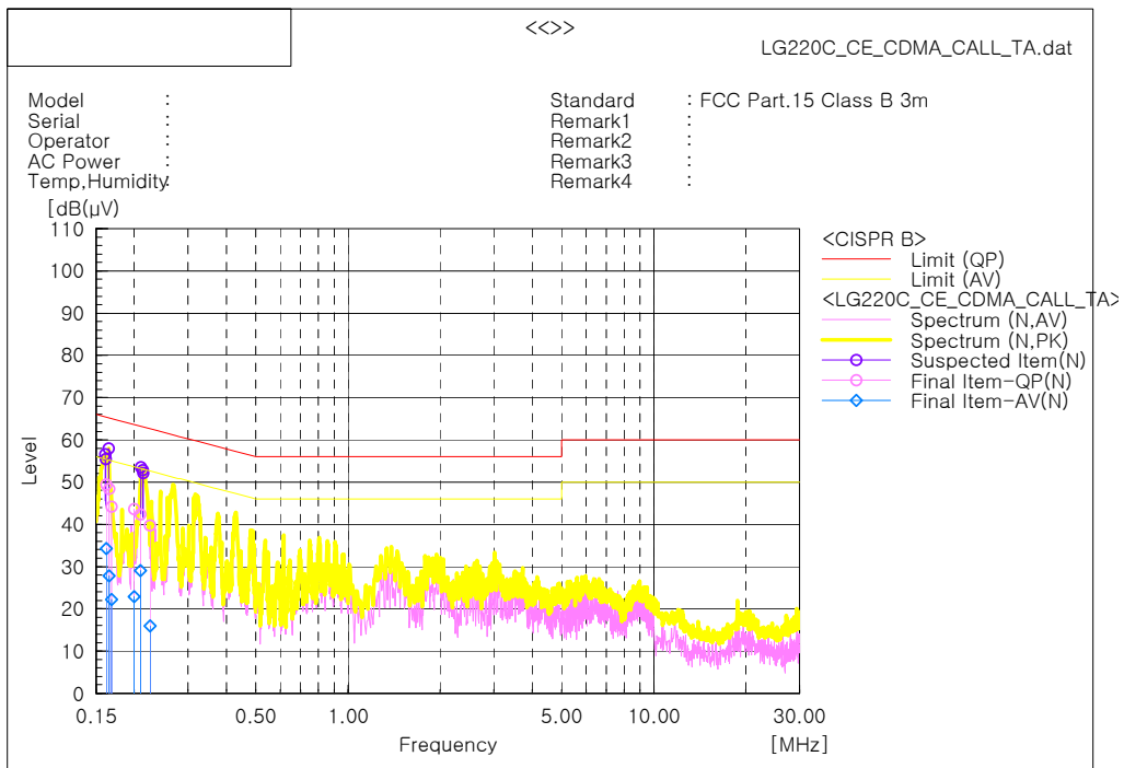
Plot 7-1. Line-Conducted Test Plot.
