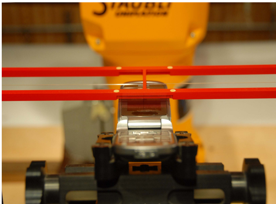
Figure 17-1 Ear Reference Point HAC Phantom Alignment
