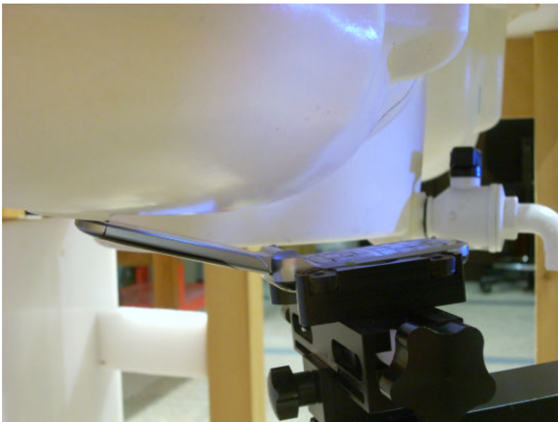
Figure 4: Right Head SAR, 15° Tilt
