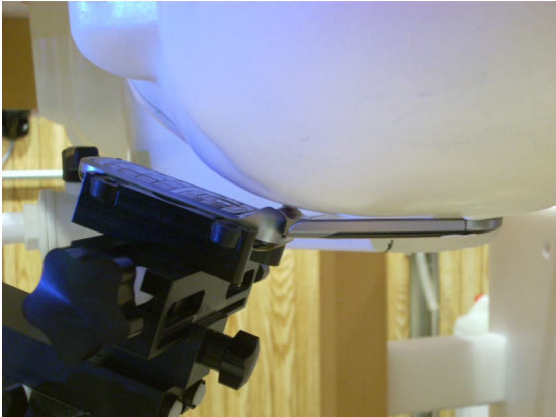
Figure 5: Left Head SAR, Cheek Touch
