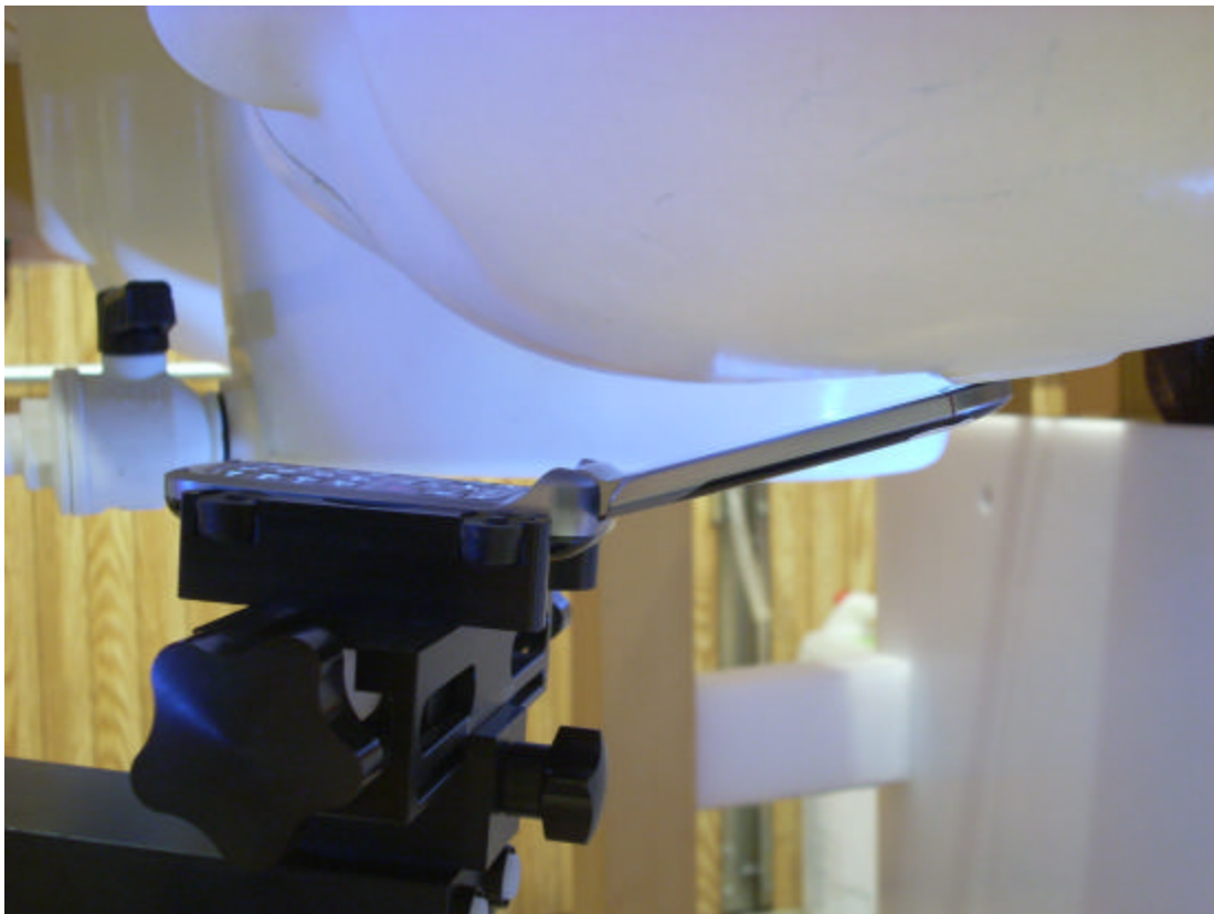
Figure 6: Left Head SAR, 15° Tilt
