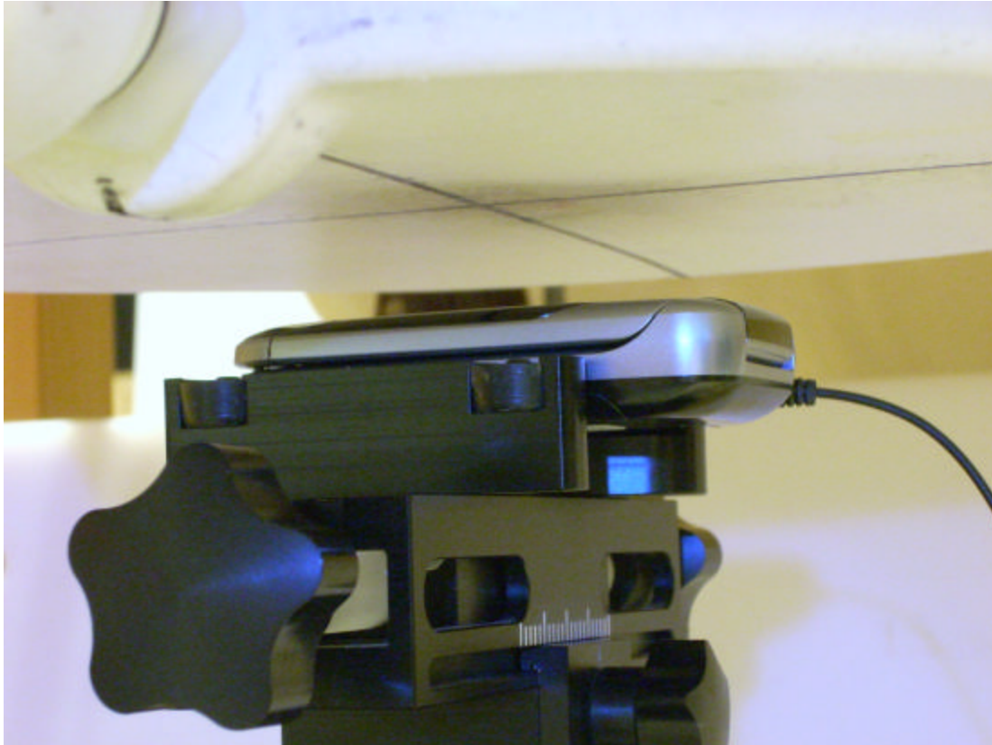
Figure 9: Body SAR, Front Side with 20mm Space
