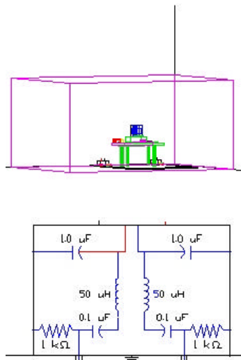
Fig. 3. LISN Schematic Diagram
