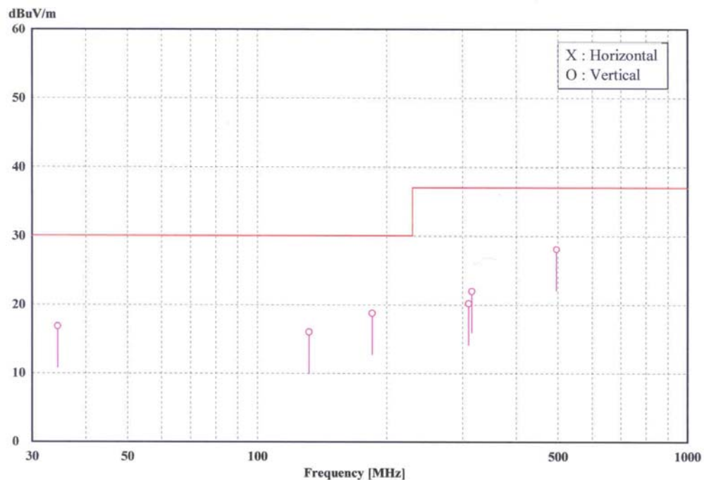
< Fig 6-2. Radiated emission result >
