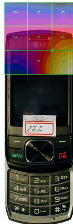
Figure 16-5 H-Field WD Scan overlay
