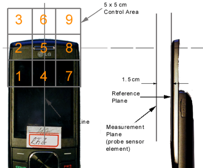
Figure 16-3 5x5 Scan grid above WD
