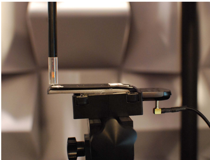
Figure 12-1 Test Setup for Wireless Device
