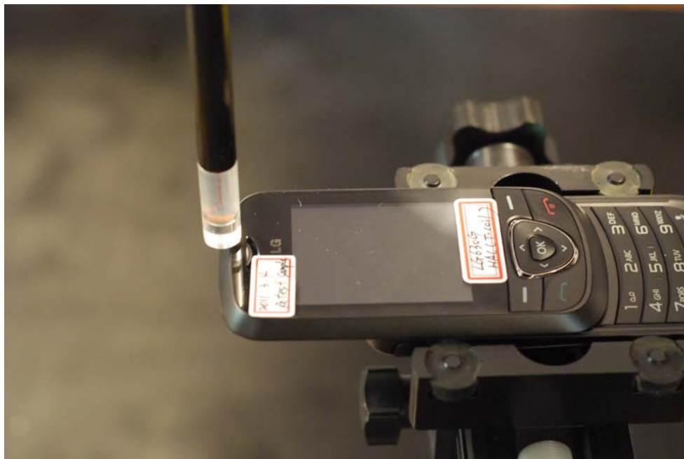
Figure 12-2 Test Setup for Wireless Device
