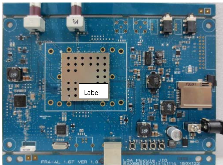
Figure 1.2 Label Location
