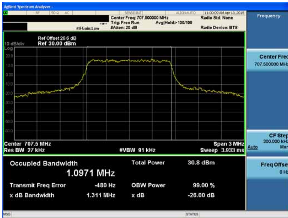
BAND 12. Occupied Bandwidth Plot (1.4M BW Ch.23095 QPSK RB 6)
