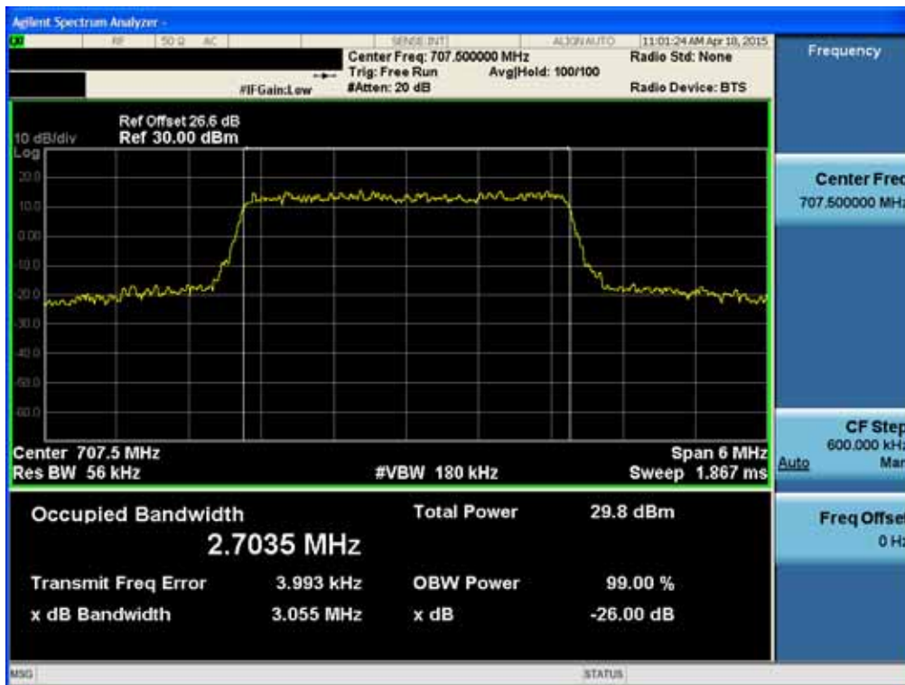
BAND 12. Occupied Bandwidth Plot (3M BW Ch.23095 16QAM RB 15)
