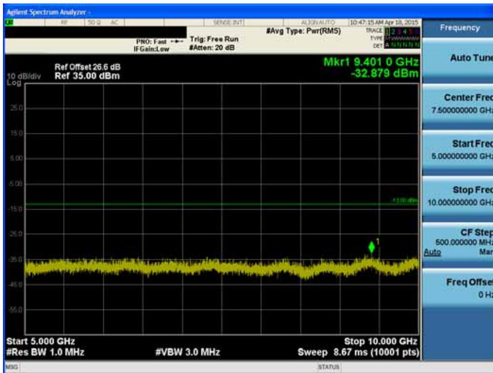
BAND 12. Conducted Spurious Plot_2 (23060ch_10MHz_QPSK_RB 1_0)
