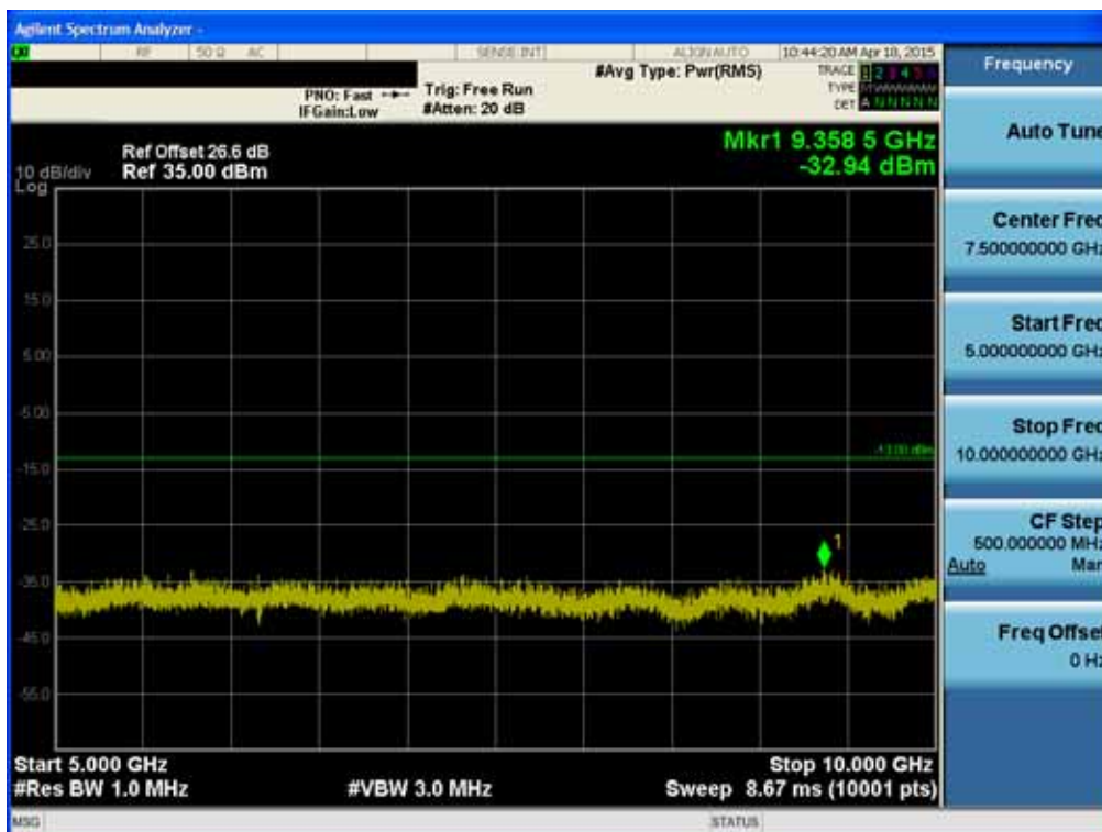
BAND 12. Conducted Spurious Plot_2 (23095ch_3MHz_QPSK_RB 1_0)
