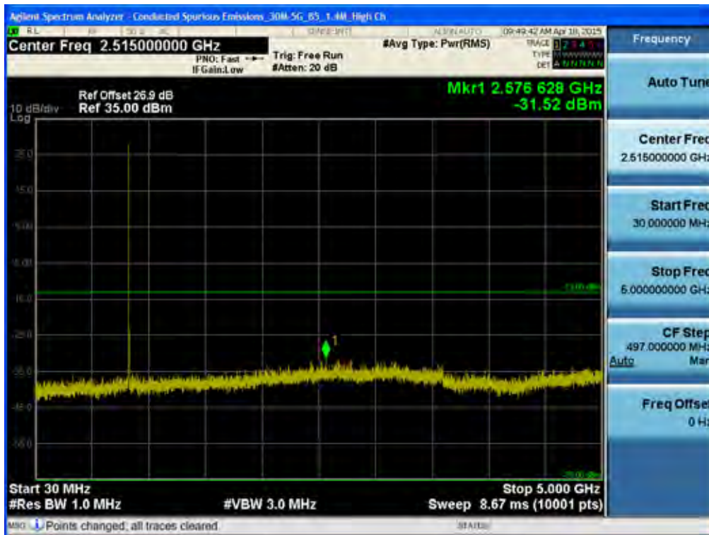
BAND 5. Conducted Spurious Plot _1 (20643ch_1.4MHz_QPSK_RB 1_0)
