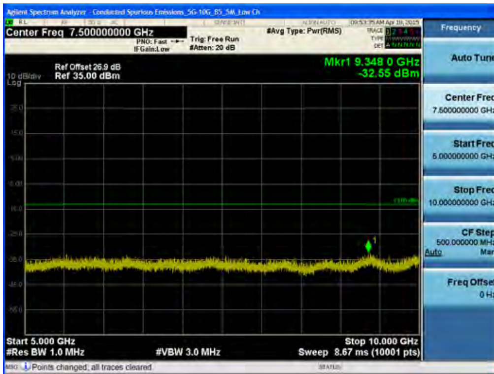
BAND 5. Conducted Spurious Plot _2 (20425ch_5MHz_QPSK_RB 1_0)
