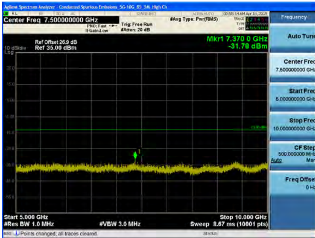
BAND 5. Conducted Spurious Plot _2 (20625ch_5MHz_QPSK_RB 1_0)
