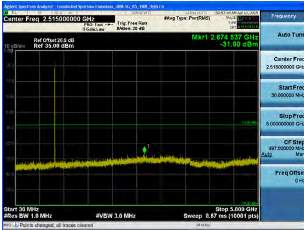
BAND 5. Conducted Spurious Plot _1 (20600ch_10MHz_QPSK_RB 1_0)
