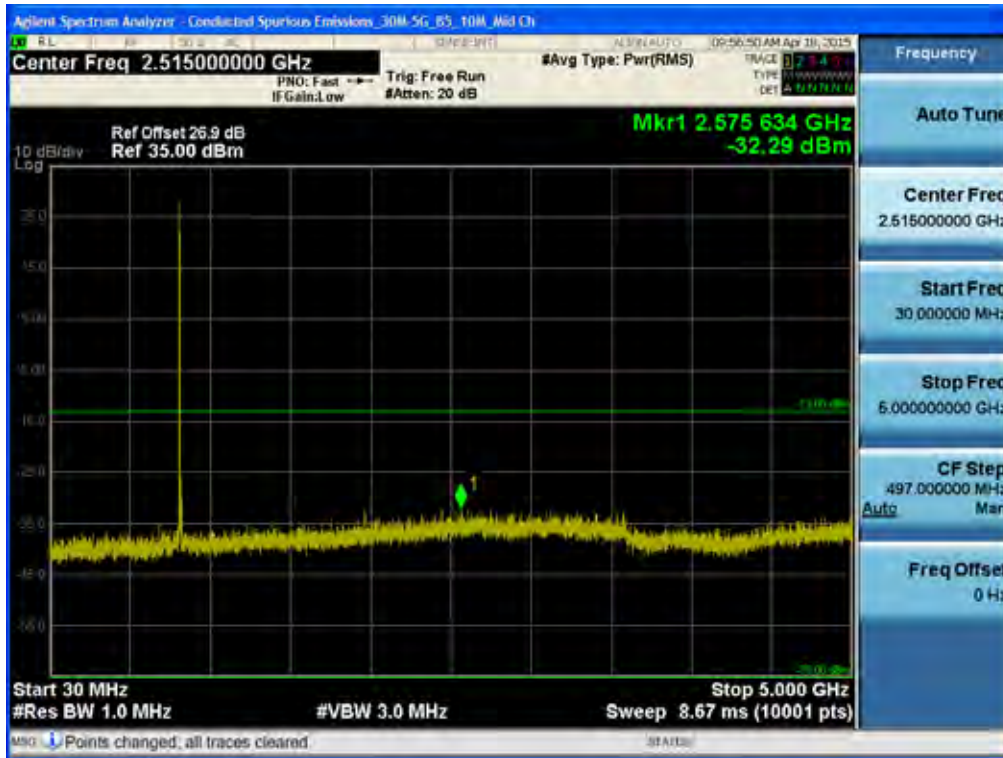
BAND 5. Conducted Spurious Plot _1 (20525ch_10MHz_QPSK_RB 1_0)
