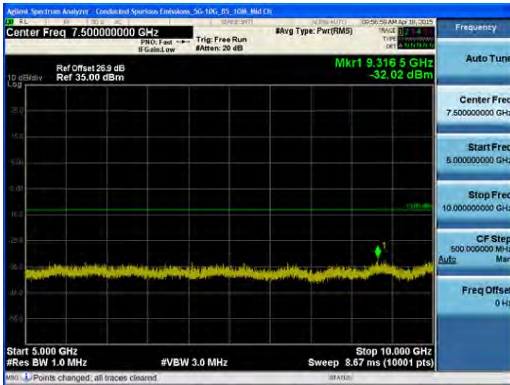
BAND 5. Conducted Spurious Plot _2 (20525ch_10MHz_QPSK_RB 1_0)
