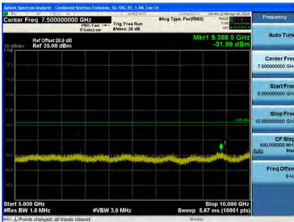
BAND 5. Conducted Spurious Plot _2 (20407ch_1.4MHz_QPSK_RB 1_0)
