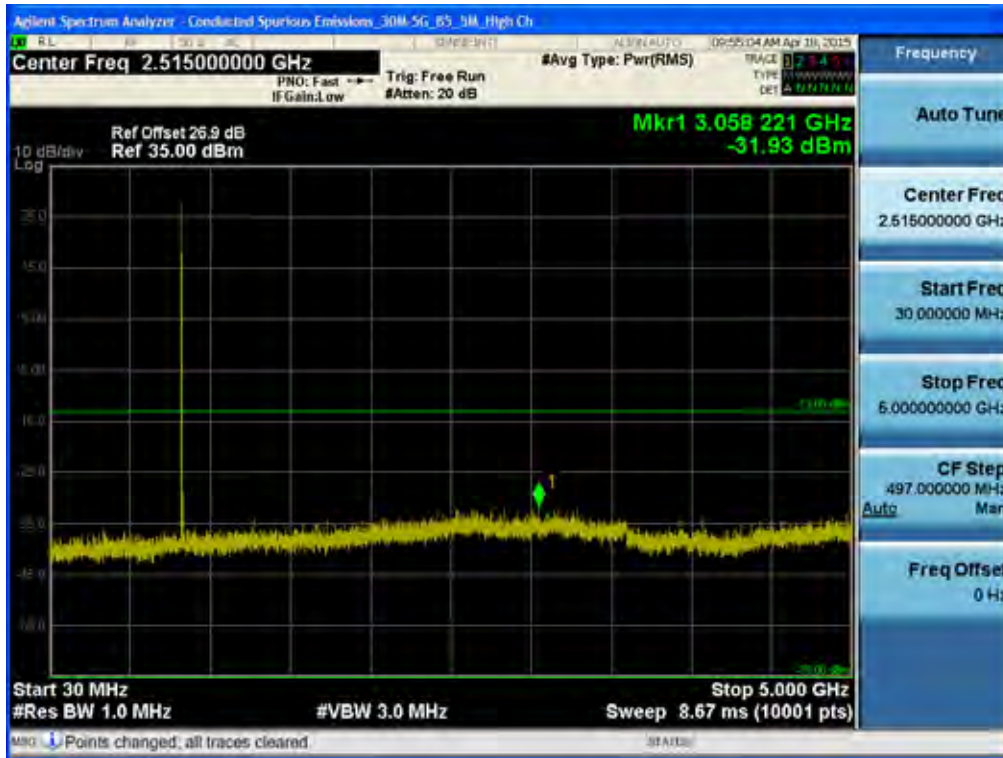
BAND 5. Conducted Spurious Plot _1 (20625ch_5MHz_QPSK_RB 1_0)
