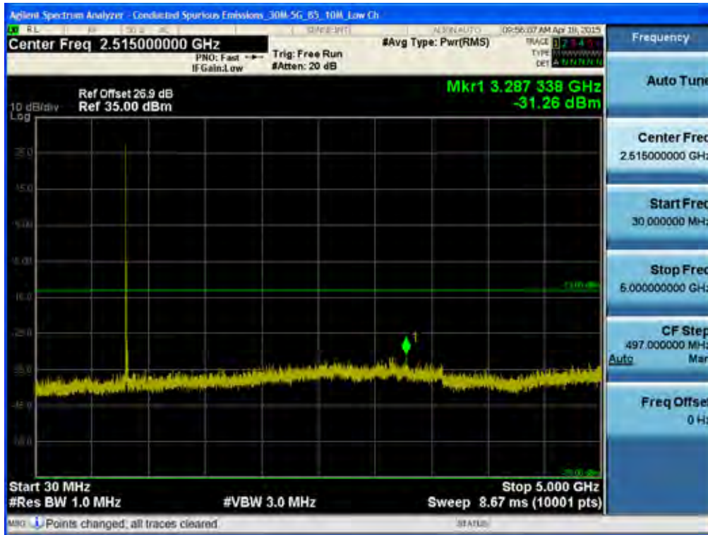
BAND 5. Conducted Spurious Plot _1 (20450ch_10MHz_QPSK_RB 1_0)
