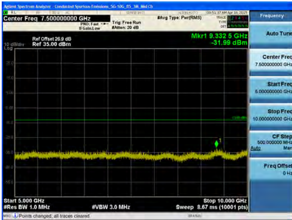
BAND 5. Conducted Spurious Plot _2 (20525ch_3MHz_QPSK_RB 1_0)
