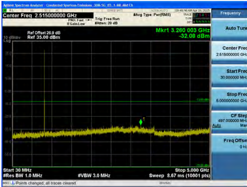
BAND 5. Conducted Spurious Plot _1 (20525ch_1.4MHz_QPSK_RB 1_0)
