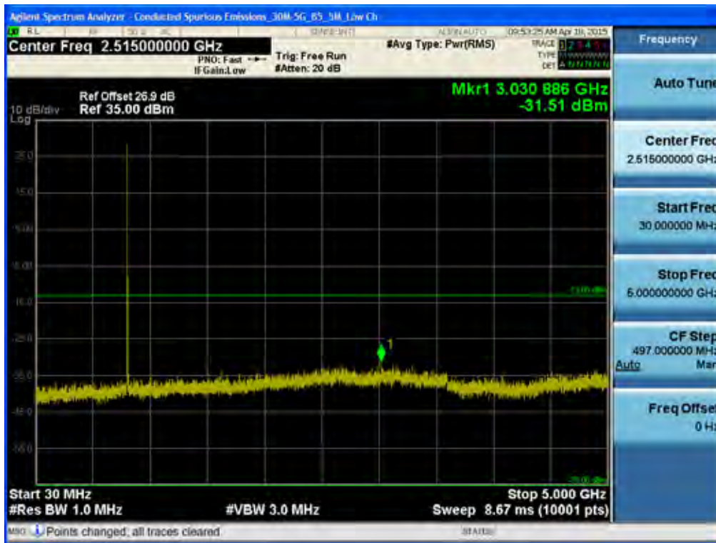
BAND 5. Conducted Spurious Plot _1 (20425ch_5MHz_QPSK_RB 1_0)
