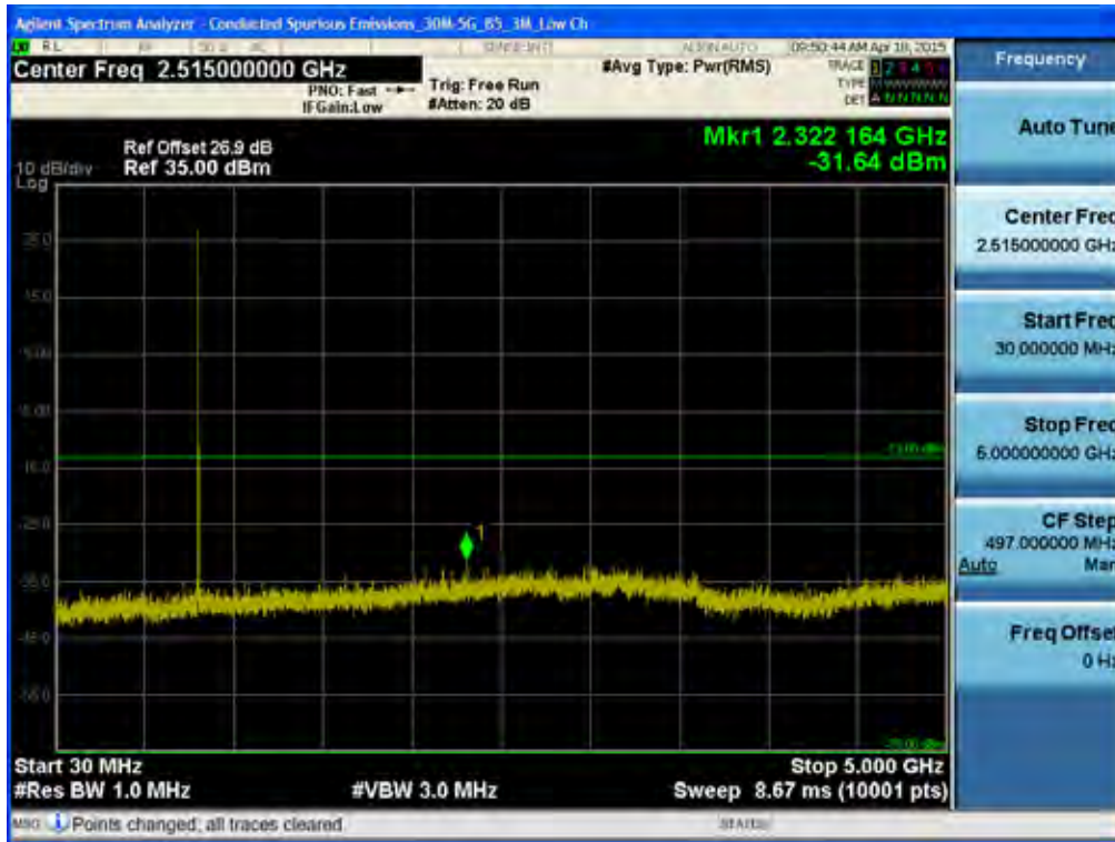
BAND 5. Conducted Spurious Plot _1 (20415ch_3MHz_QPSK_RB 1_0)
