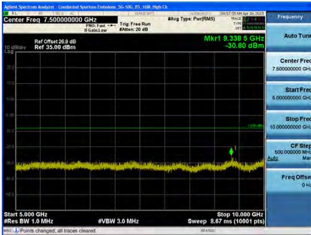
BAND 5. Conducted Spurious Plot _2 (20600ch_10MHz_QPSK_RB 1_0)
