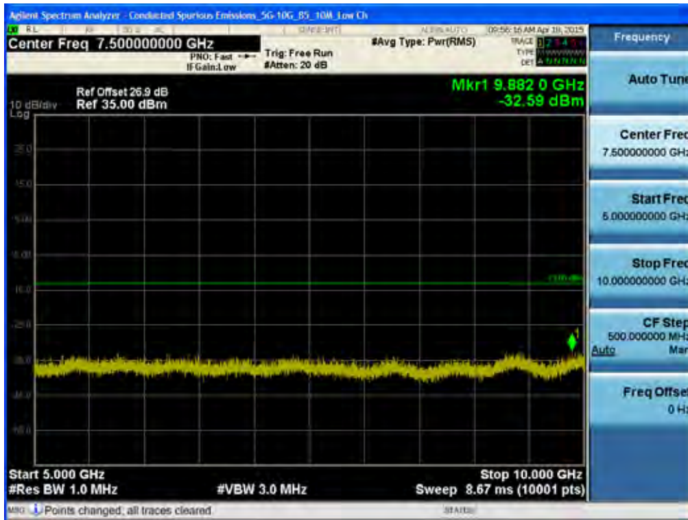
BAND 5. Conducted Spurious Plot _2 (20450ch_10MHz_QPSK_RB 1_0)
