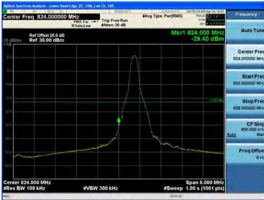
BAND 5. Lower Band Edge Plot (10M BW Ch.20450 QPSK_RB1_Offset 0)
