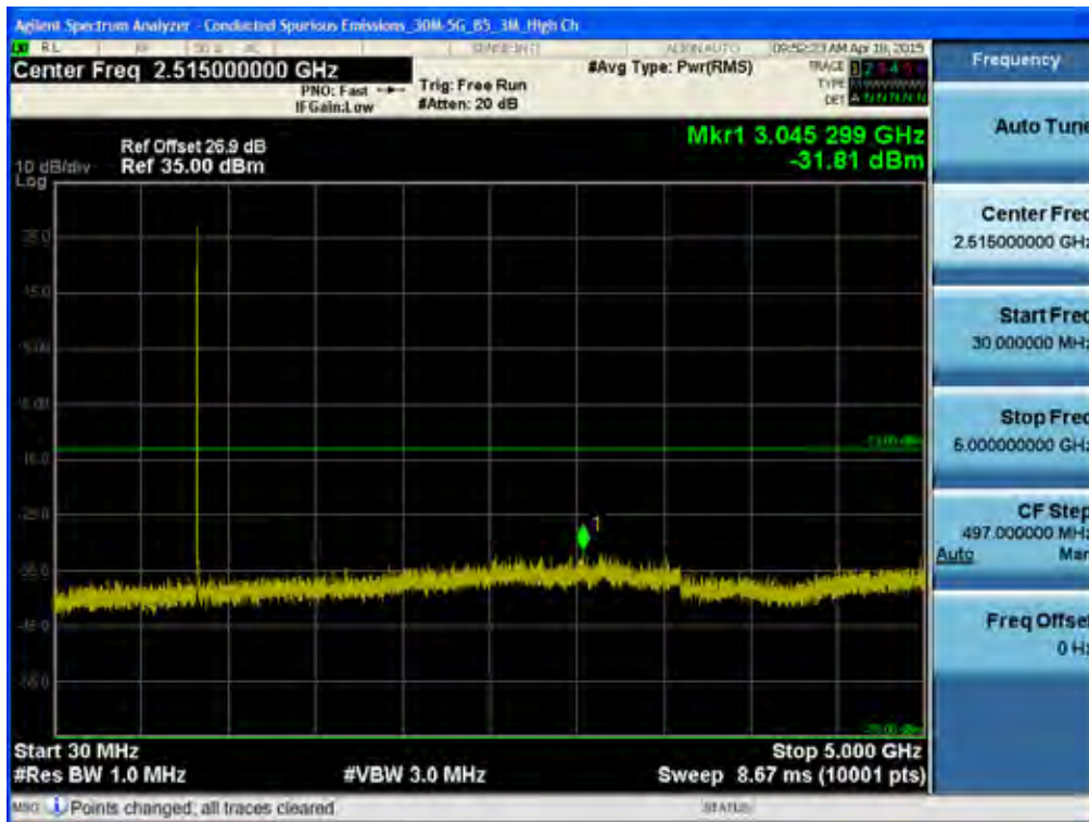
BAND 5. Conducted Spurious Plot _1 (20635ch_3MHz_QPSK_RB 1_0)
