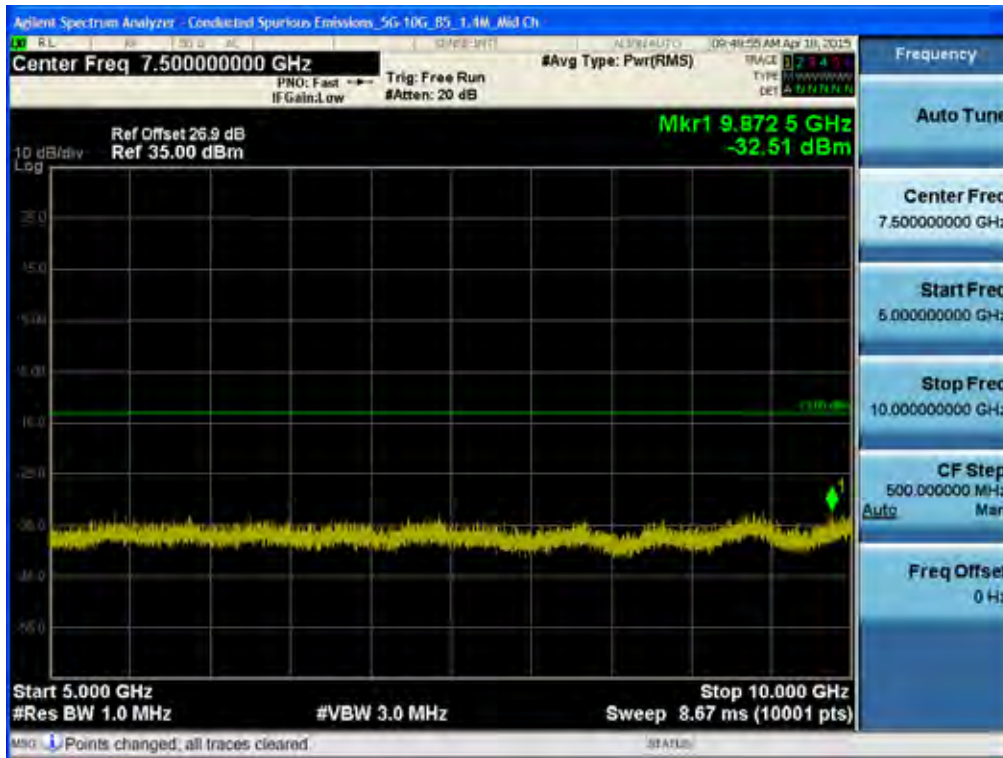
BAND 5. Conducted Spurious Plot _2 (20525ch_1.4MHz_QPSK_RB 1_0)
