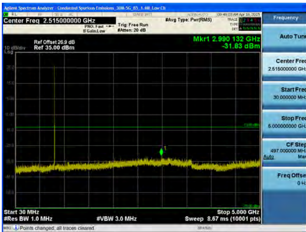
BAND 5. Conducted Spurious Plot _1 (20407ch_1.4MHz_QPSK_RB 1_0)
