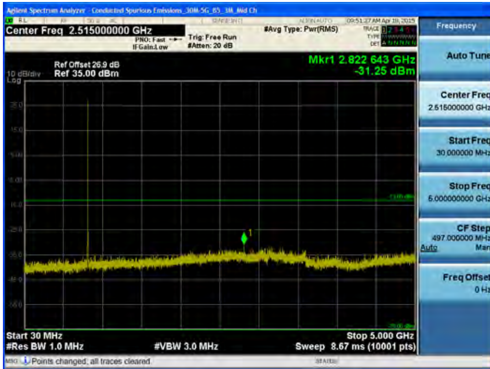
BAND 5. Conducted Spurious Plot _1 (20525ch_3MHz_QPSK_RB 1_0)
