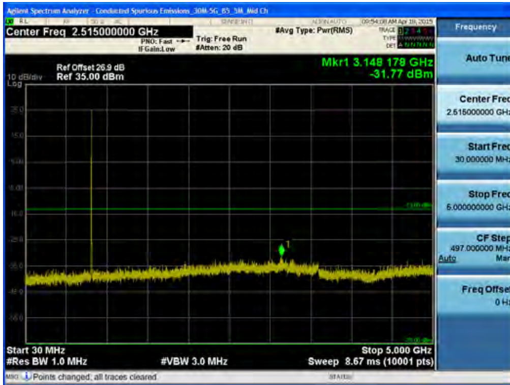
BAND 5. Conducted Spurious Plot _1 (20525ch_5MHz_QPSK_RB 1_0)
