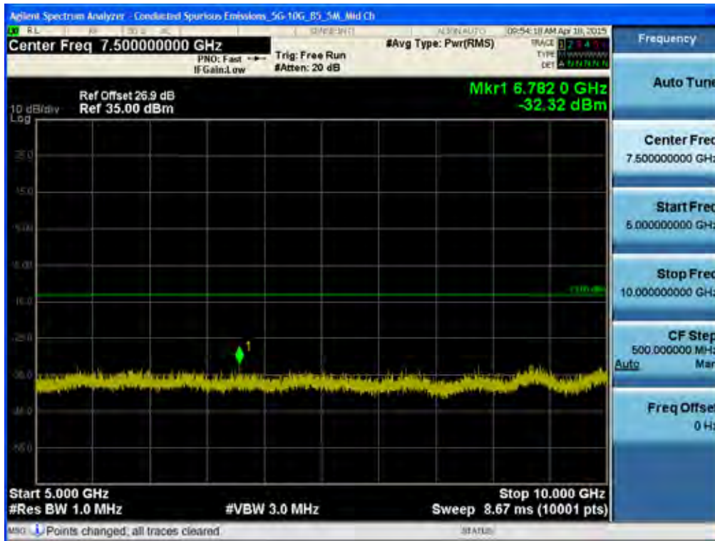
BAND 5. Conducted Spurious Plot _2 (20525ch_5MHz_QPSK_RB 1_0)
