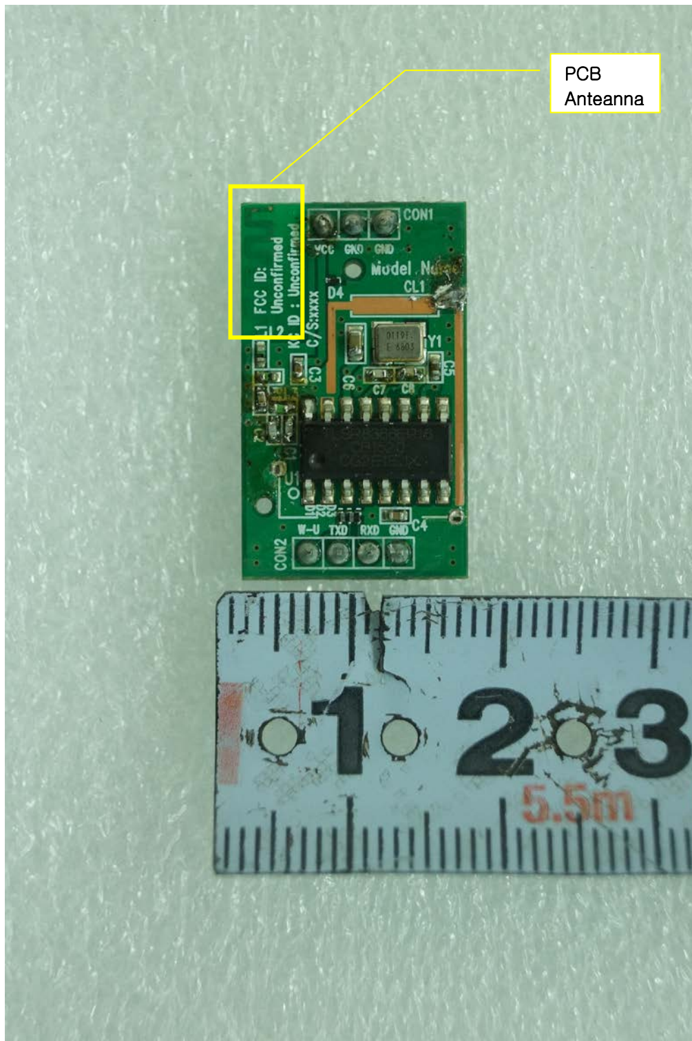
< Main board top view (removed shield) >
