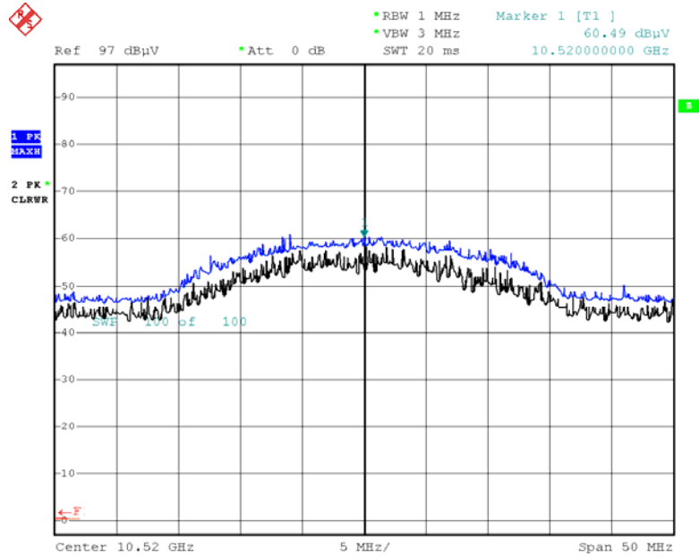
Peak Reading (802.11a, Ch.52 2nd Harmonic, Z-V)
