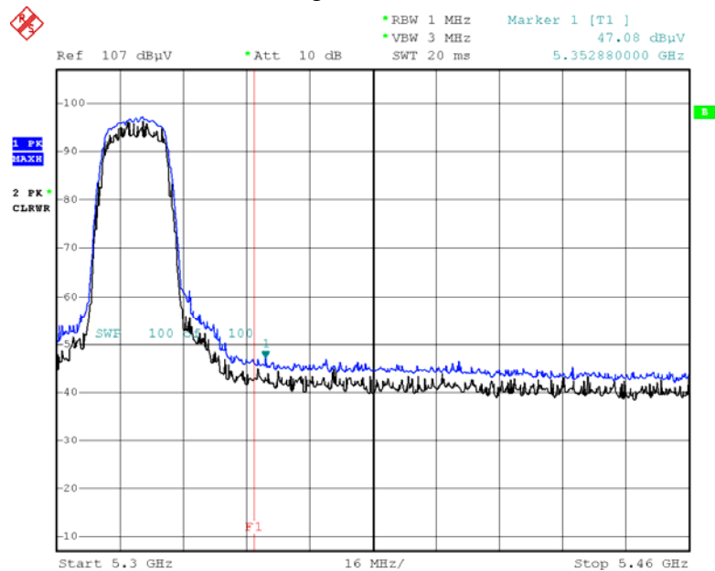
Peak Reading (802.11a, Ch.64, X-H)
