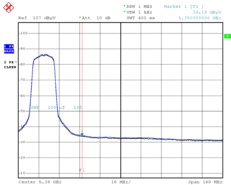
Average Reading (802.11a, Ch.64, X-H)
