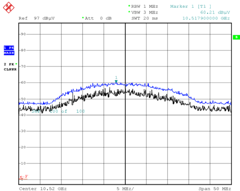
Peak Reading (802.11n(HT20), Ch.52 2nd Harmonic, Z-V)
