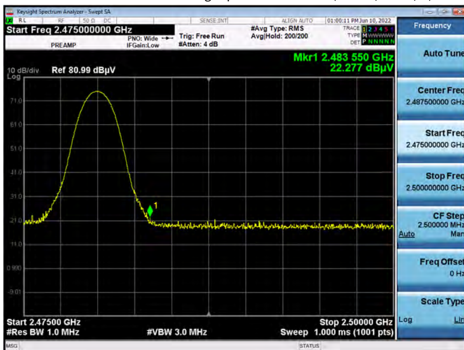
Radiated Restricted Band Edges plot –Peak Result (8DPSK, Ch.78, H)
