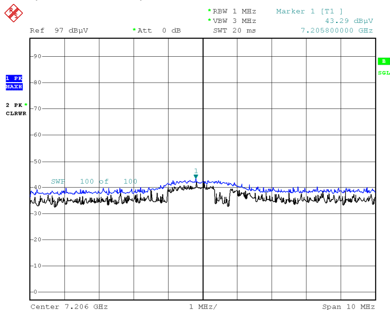
Radiated Spurious Emissions plot – Peak Result (GFSK, Ch.0 3rd Harmonic, X-H)
