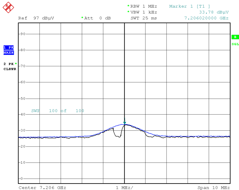
Radiated Spurious Emissions plot – Average Result (GFSK, Ch.0 3rd Harmonic, X-H)
