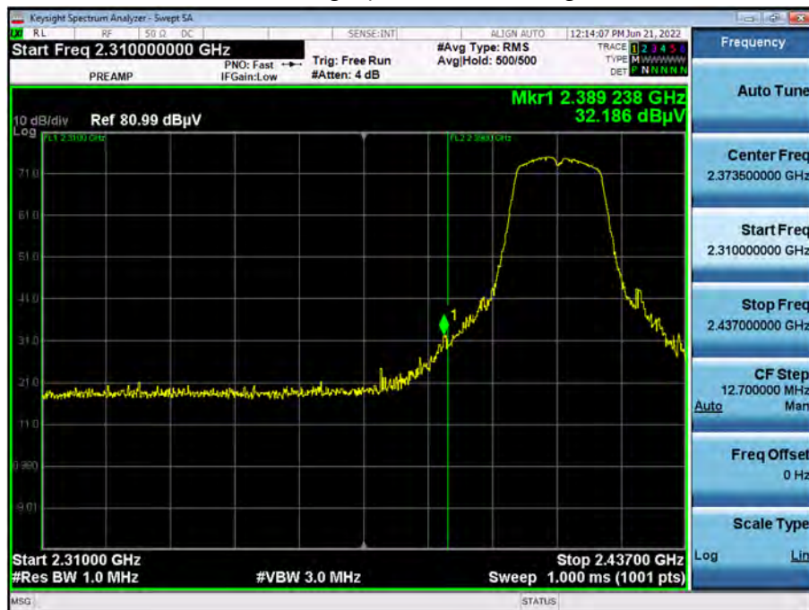
Radiated Restricted Band Edges plot – Peak Reading (802.11n Ch.01, Z-H)
