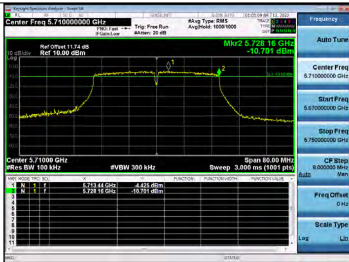
802.11ac_VHT40 CH.142
