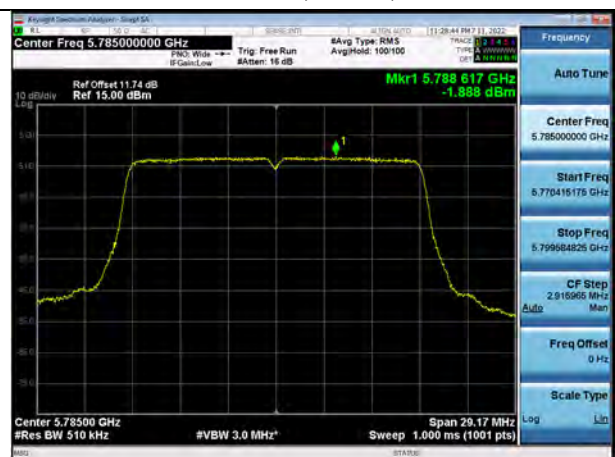
UNII 3 (Ch. 157)
