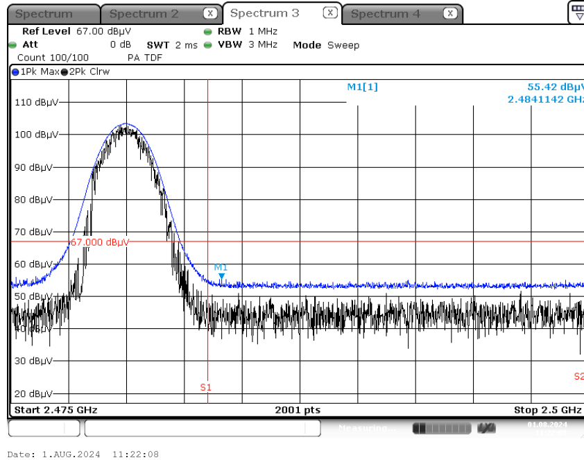
Radiated Restricted Band Edges plot – Average &amp; Peak Result (8DPSK, Ch. 78, Y-V)
