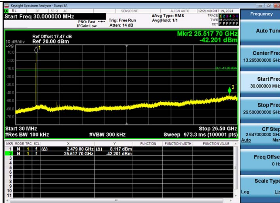
Spurious Emission (30 MHz – 26.50 GHz) 8DPSK, CH. 78
