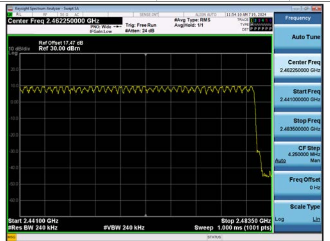
\pi/4 DQPSK Number of Channels (2.441 GHz - 2.483.5 GHz)
