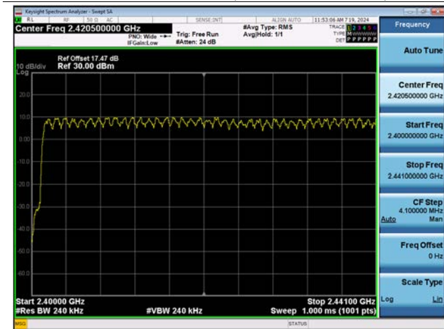
\pi/4 DQPSK Number of Channels (2.4 GHz - 2.441 GHz)
