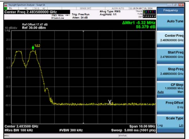
GFSK Band Edge(CH.78)
