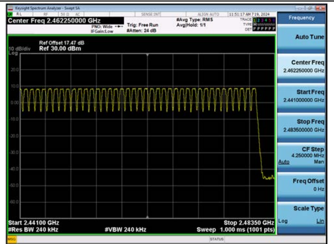
8DPSK Number of Channels (2.441 GHz - 2.483.5 GHz)
