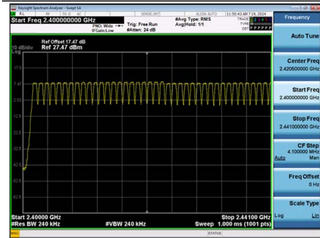
8DPSK Number of Channels (2.4 GHz - 2.441 GHz)
