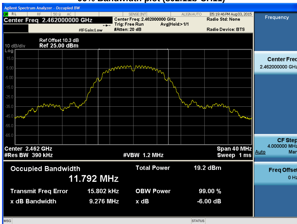
99% Bandwidth plot (802.11b-CH11)
