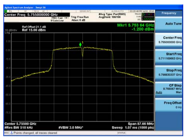
802.11ac_VHT40 UNII 3 BAND PSD CH 151
