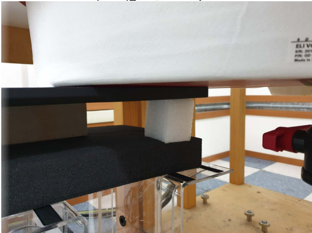
SAR Test Picture(Front)_Aux, Test separation distance : 0 mm
