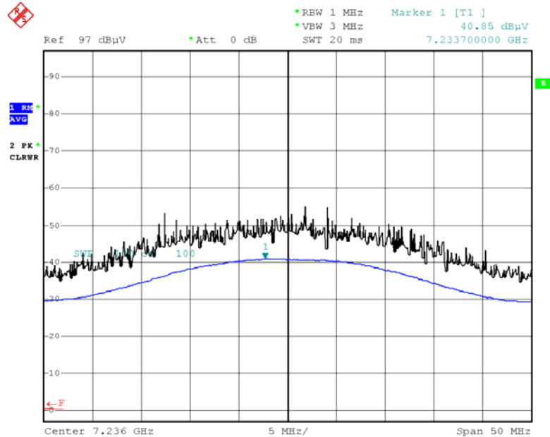
Radiated Spurious Emissions plot – Average Reading (802.11n (HT20), Ch.1 3rd Harmonic)
