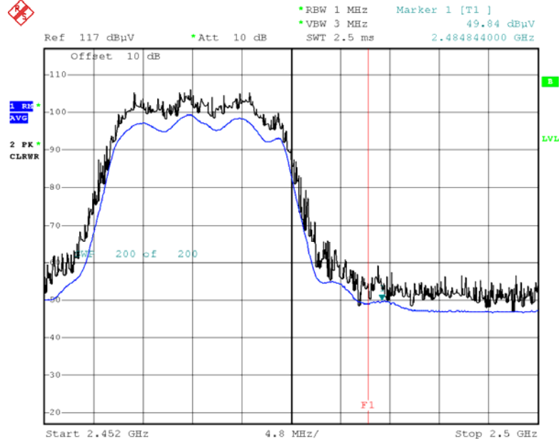
Radiated Restricted Band Edges plot – Average Reading (802.11g Ch.12)
