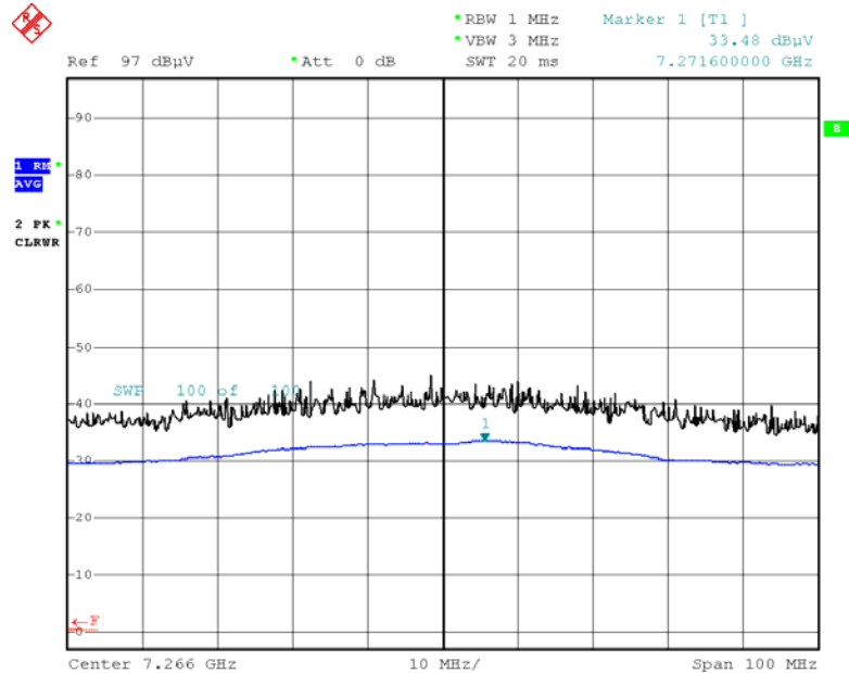
Radiated Spurious Emissions plot – Average Reading (802.11n (HT40), Ch.3 3rd Harmonic)
