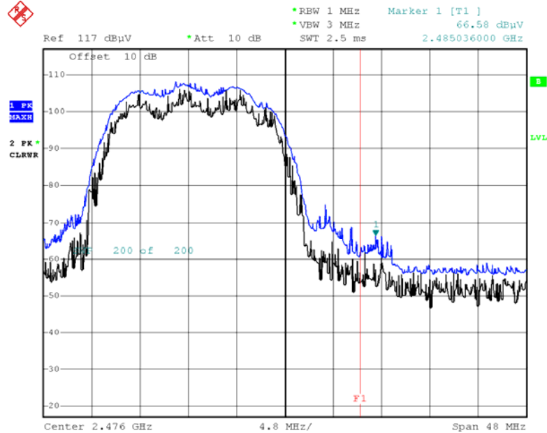
Radiated Restricted Band Edges plot – Peak Reading (802.11g Ch.12)
