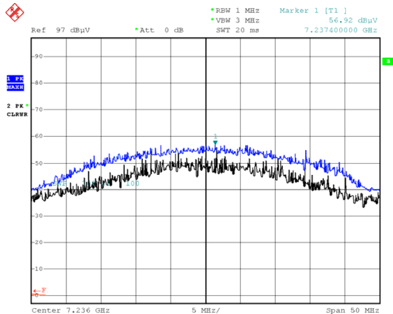
Radiated Spurious Emissions plot – Peak Reading (802.11n (HT20), Ch.1 3rd Harmonic)
