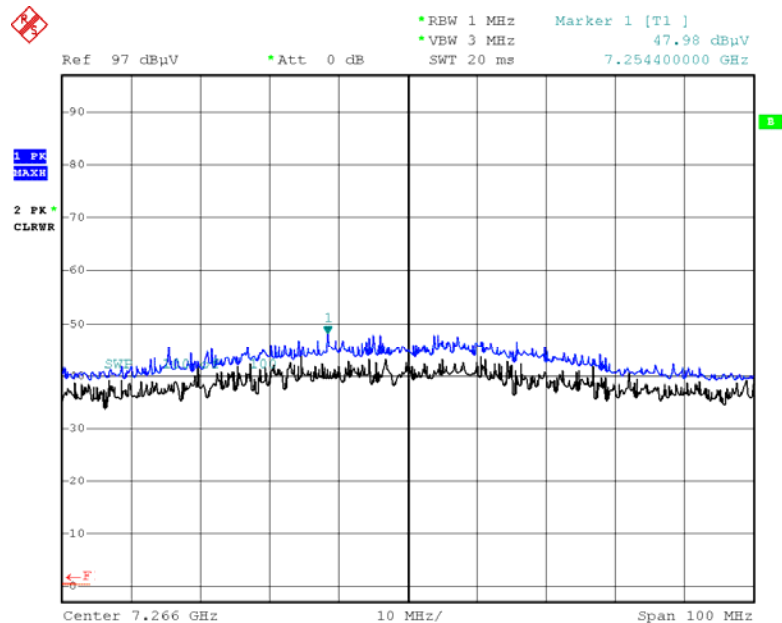
Radiated Spurious Emissions plot – Peak Reading (802.11n (HT40), Ch.3 3rd Harmonic)
