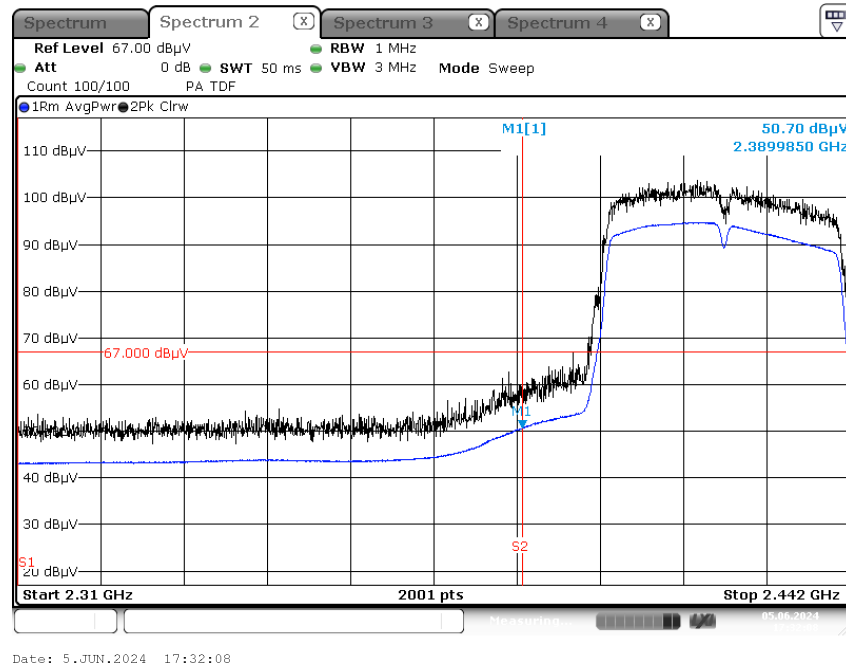
Radiated Restricted Band Edges plot - Average Reading (802.11n(HT40), Ch. 3, Z-V)
