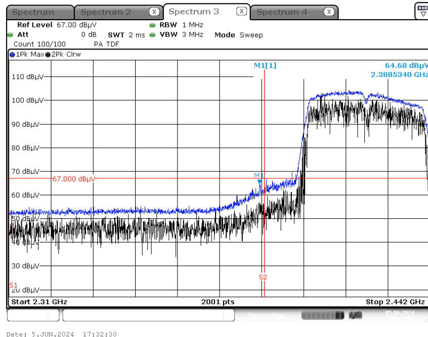
Radiated Restricted Band Edges plot - Peak Reading (802.11n(HT40), Ch. 3, Z-V)
