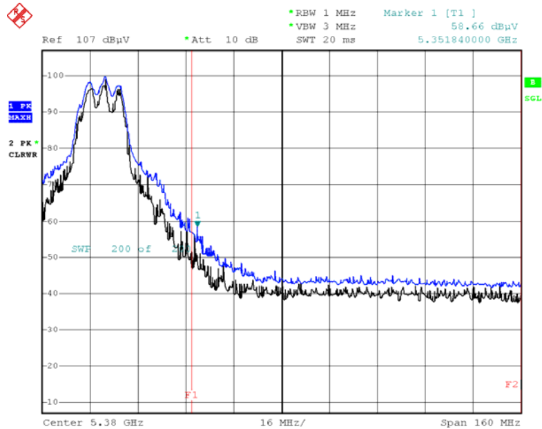
Peak Reading (802.11a, Ch.64)
