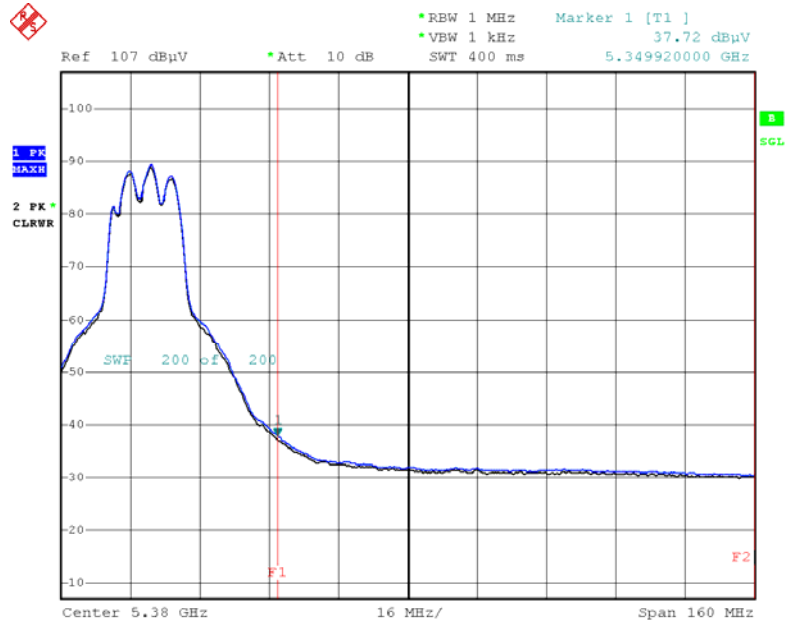
Average Reading (802.11a, Ch.64)
