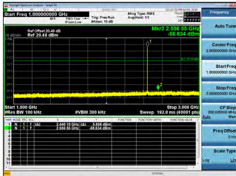
Conducted Spurious Emission (Mid-CH 19)
