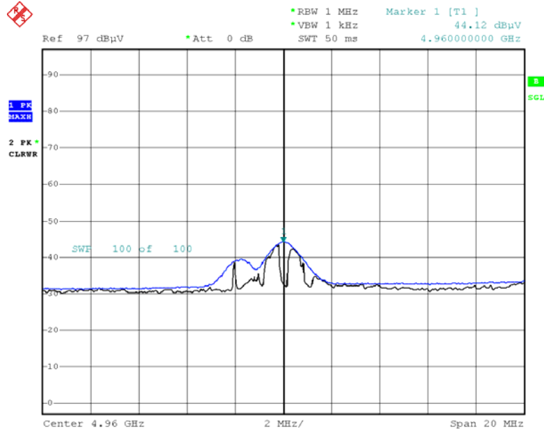
Radiated Spurious Emissions plot – Average Reading (8DPSK, Ch.78 2nd Harmonic, H)
