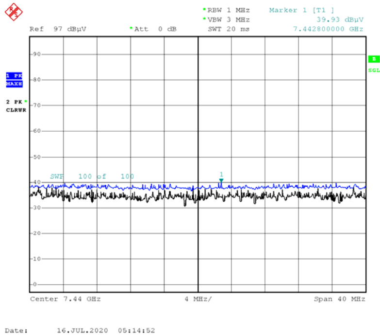
Radiated Spurious Emissions plot – Peak Reading (GFSK, Ch.78 3rd Harmonic, X-V)
