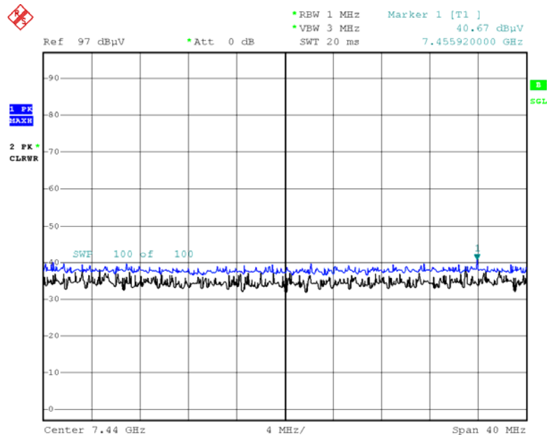
Radiated Spurious Emissions plot – Peak Reading ( \pi/4 DQPSK, Ch.78 3rd Harmonic, Y-V)
