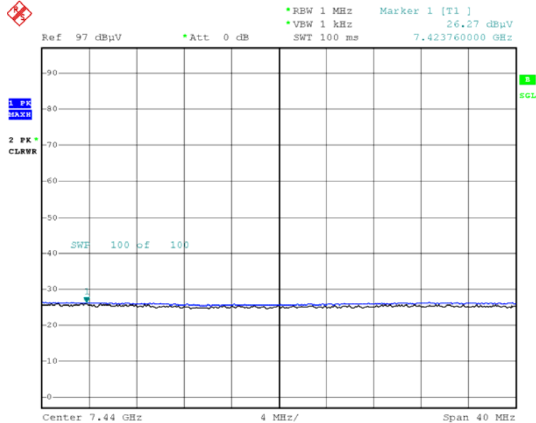
Radiated Spurious Emissions plot – Average Reading (8DPSK, Ch.78 3rd Harmonic, Y-V)
