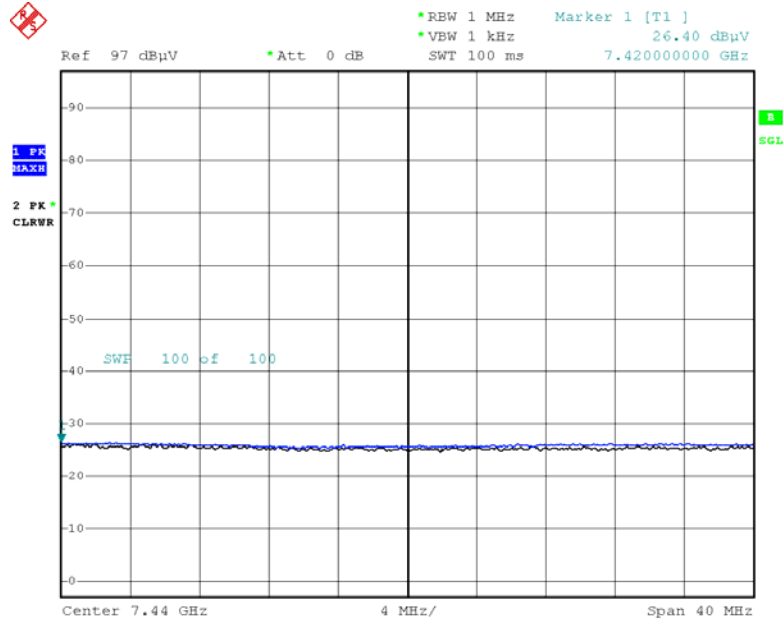
Radiated Spurious Emissions plot – Average Reading (GFSK, Ch.78 3rd Harmonic, X-V)
