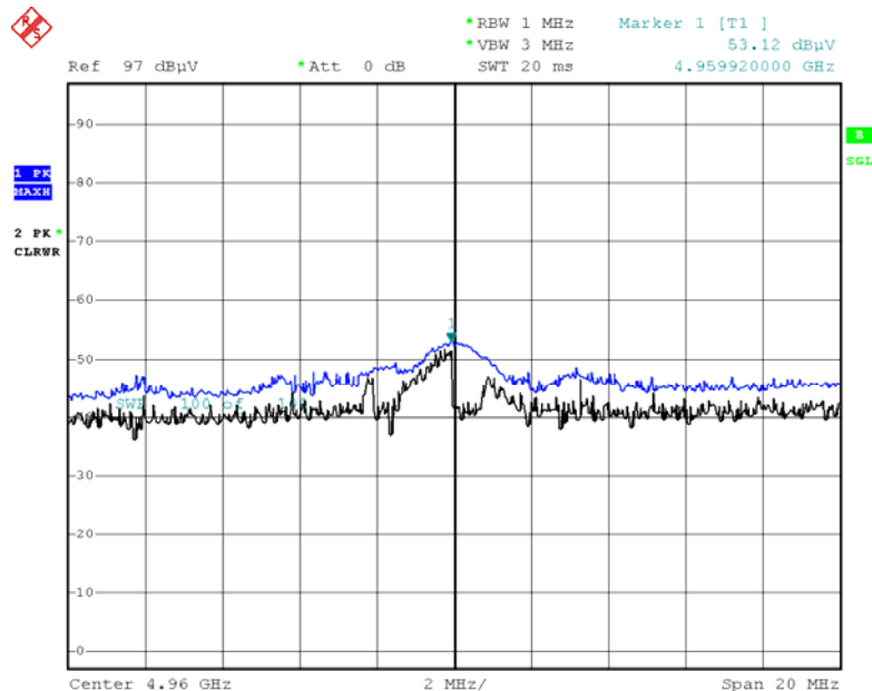
Radiated Spurious Emissions plot – Peak Reading (8DPSK, Ch.78 2nd Harmonic, H)
