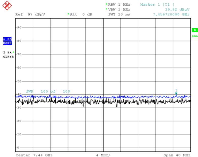
Radiated Spurious Emissions plot – Peak Reading (8DPSK, Ch.78 3rd Harmonic, Y-V)
