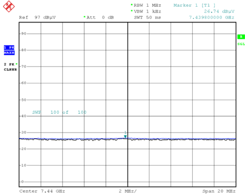
Radiated Spurious Emissions plot – Average Reading (8DPSK, Ch.78 3rd Harmonic, X-H)
