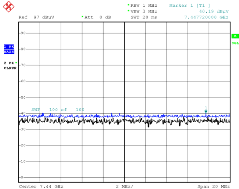
Radiated Spurious Emissions plot – Peak Reading (8DPSK, Ch.78 3rd Harmonic, X-H)
