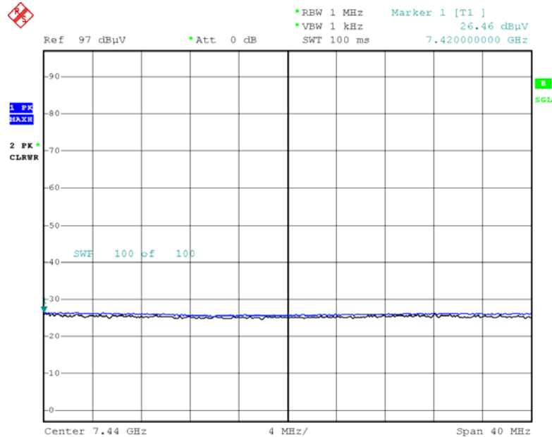
Radiated Spurious Emissions plot – Average Reading ( \pi/4 DQPSK, Ch.78 3rd Harmonic, Y-V)
