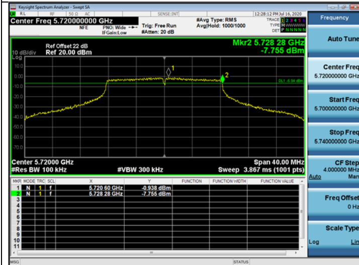
802.11ac_VHT20 CH.144
