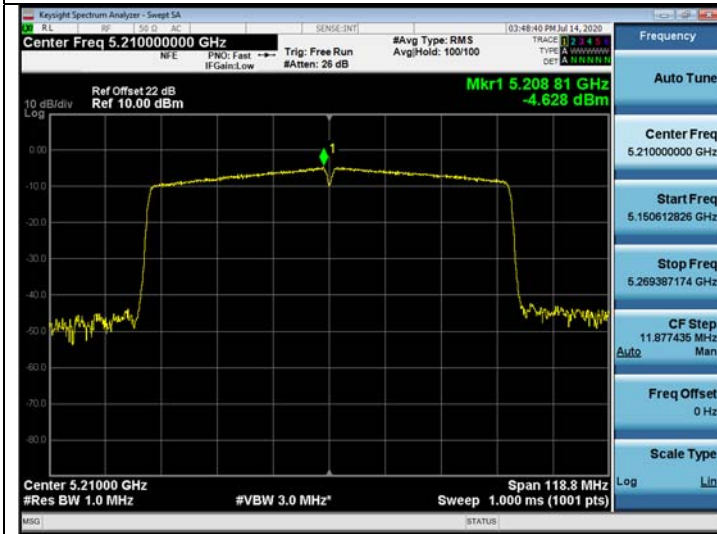
UNII 1 (Ch. 42)
