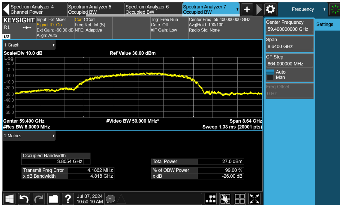
Occupied Channel Bandwidth plot (CH 9)
