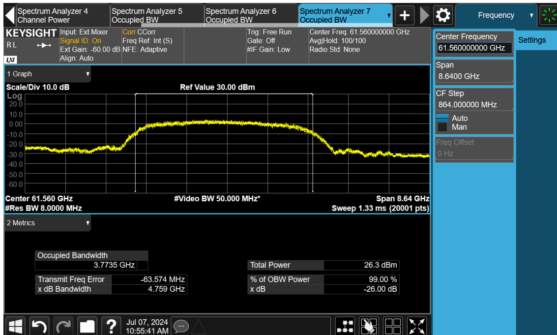
Occupied Channel Bandwidth plot (CH 10)
