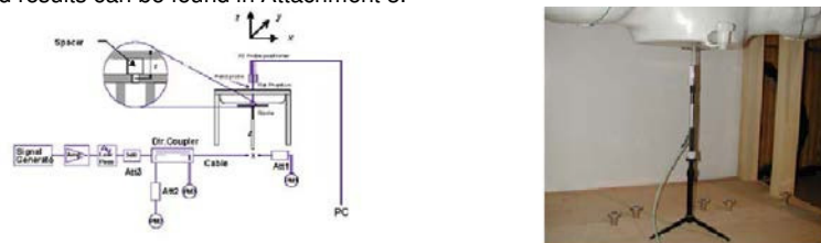
Figure 9.1 Dipole Verification Test Setup Diagram & Photo
