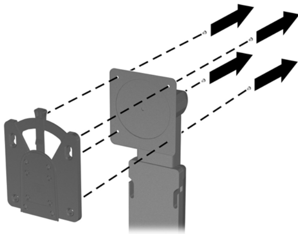
Removing the Quick Release Plate from the Pedestal Base
