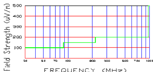
Figure 10. Limits at 3 meters
