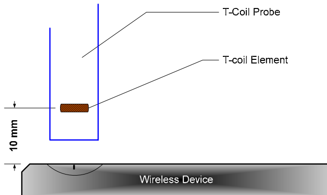
Figure 5-11 Measurement Distance
