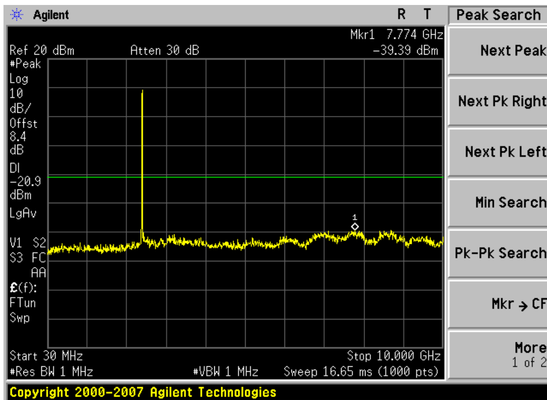
Plot 6-11. Conducted Spurious Plot (802.11b – Ch. 1)
