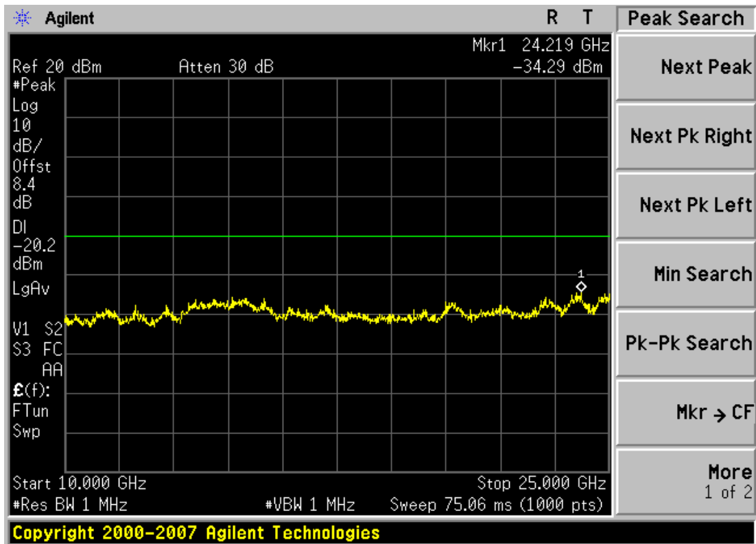
Plot 6-16. Conducted Spurious Plot (802.11b – Ch. 11)
