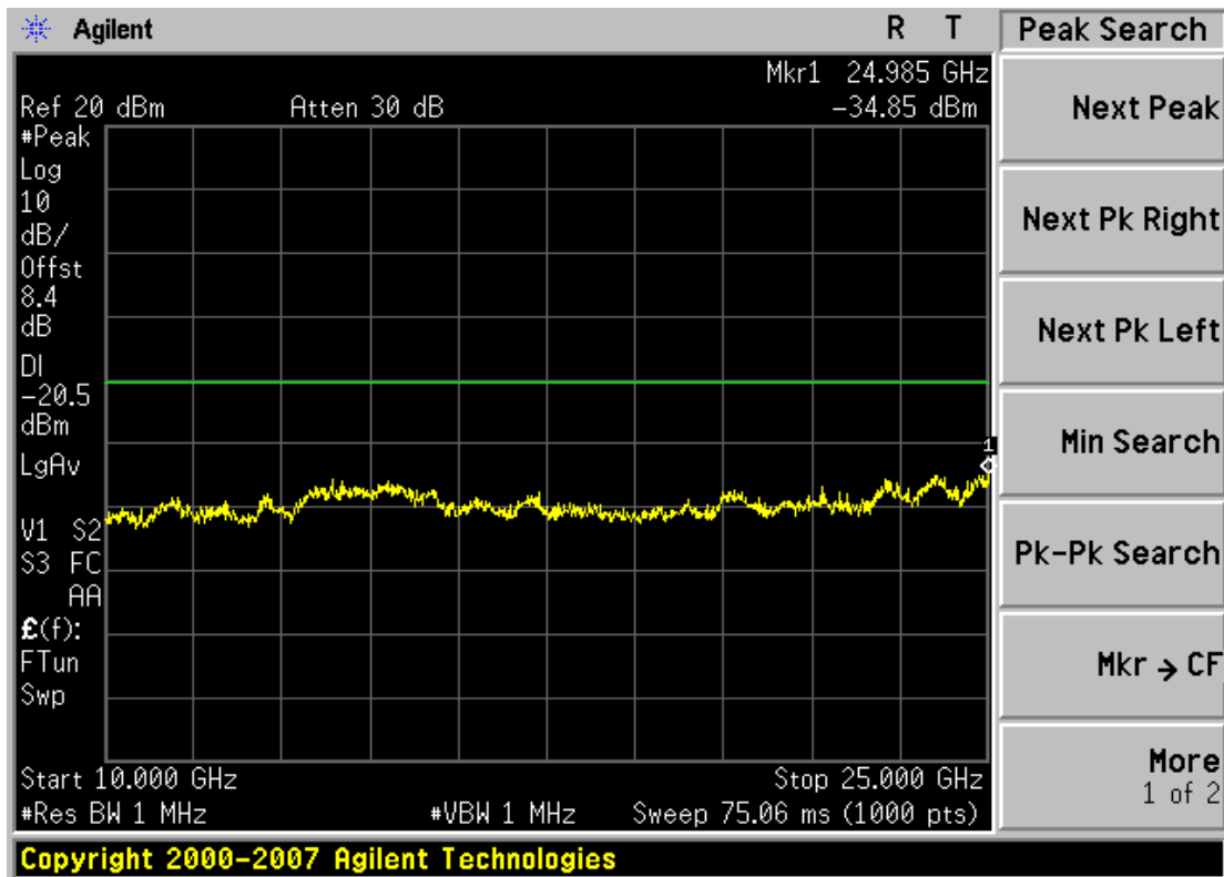
Plot 6-14. Conducted Spurious Plot (802.11b – Ch. 6)
