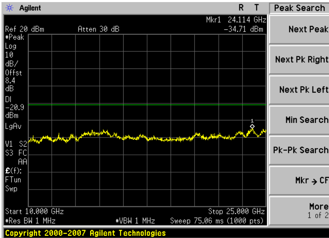
Plot 6-12. Conducted Spurious Plot (802.11b – Ch. 1)
