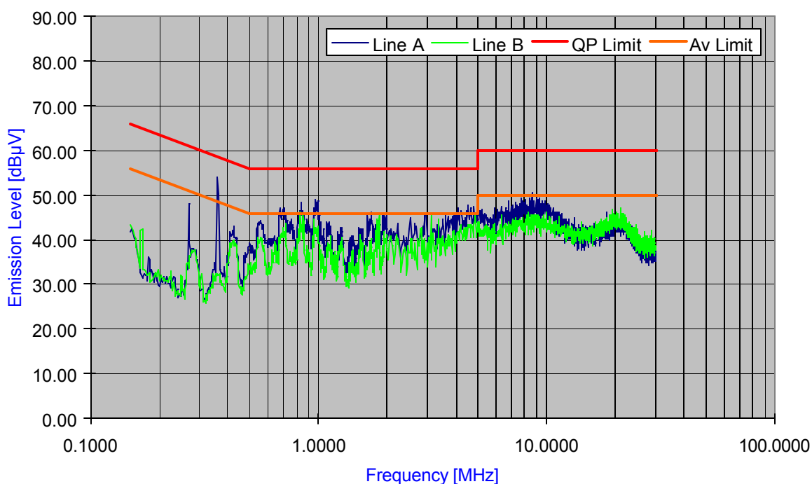
Plot 6-17. Line Conducted Plot with 802.11b
