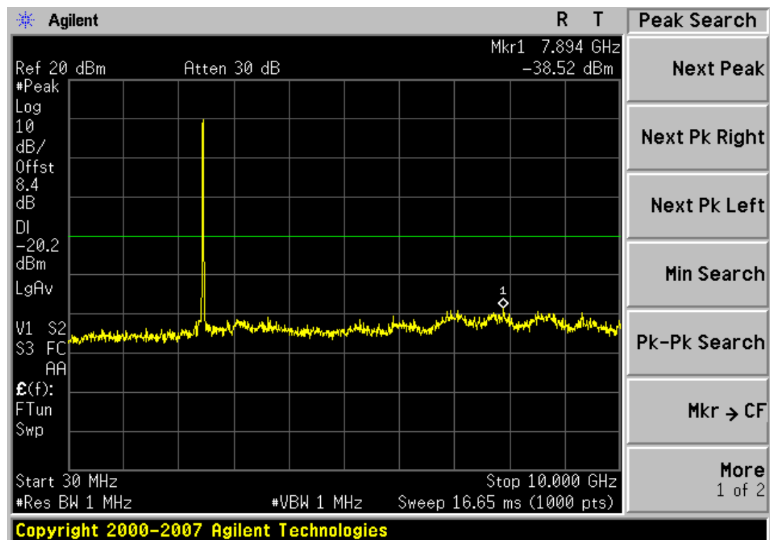
Plot 6-15. Conducted Spurious Plot (802.11b – Ch. 11)
