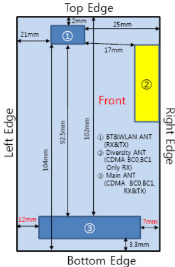
Figure 13-1 Identification of Sides for SAR Testing
